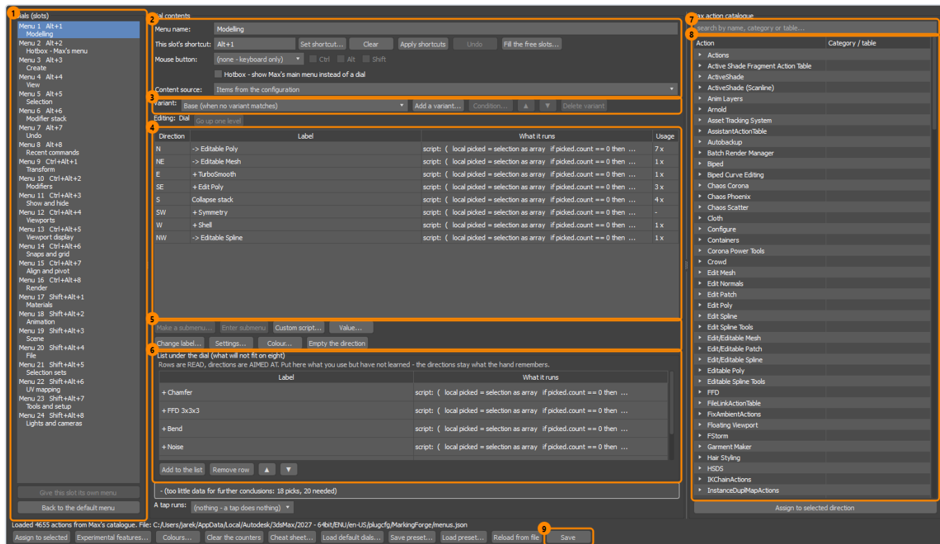
The menu editor: dials, directions, and the catalogue of every 3ds Max command.
