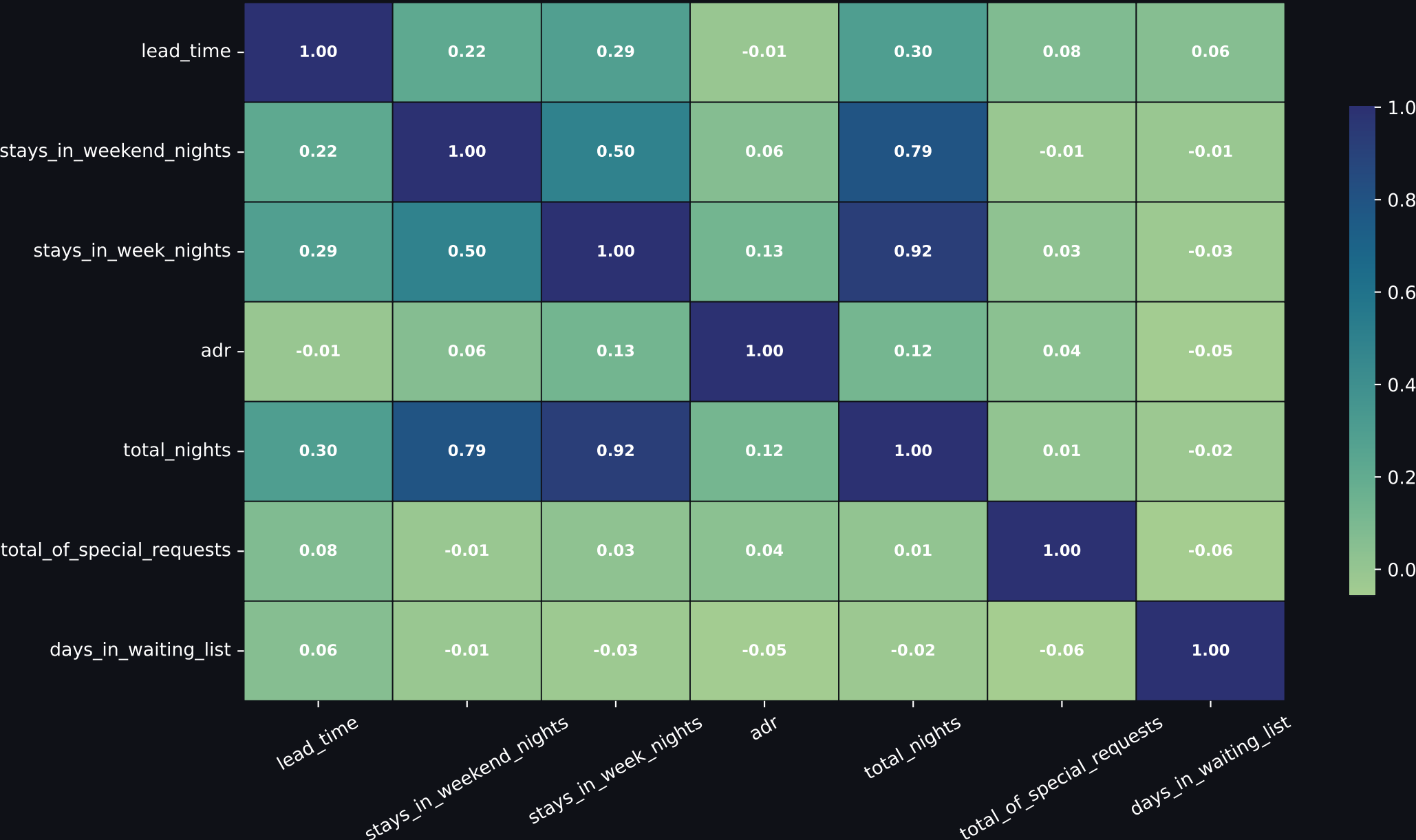
Correlation Heatmap
