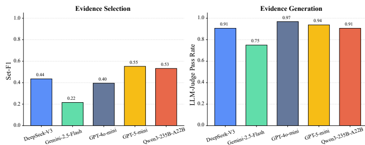
Figure 5: Evaluation of LLM performance on evidence tasks in SafeDrug.
