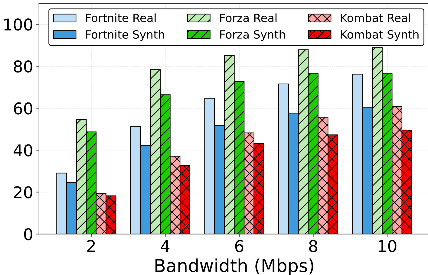
VMAF Score
