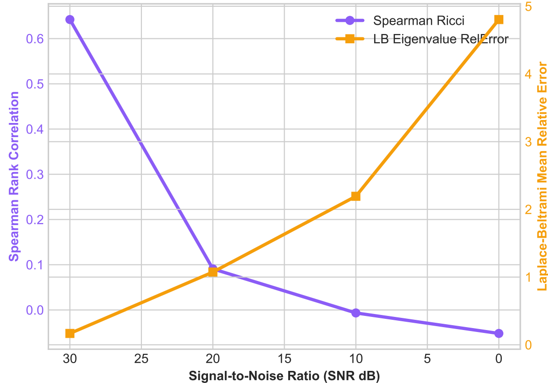
Manifold Geometrical Stability
