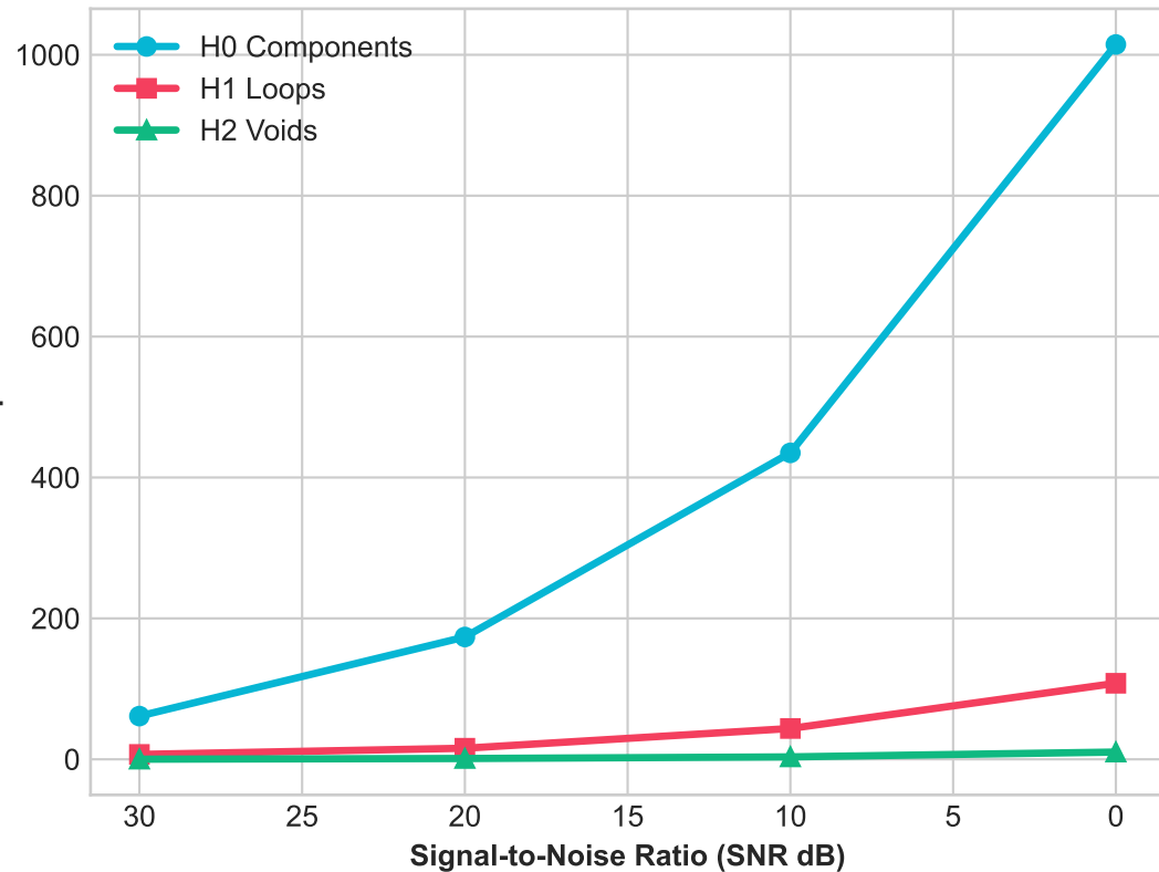
Topological Stability (TDA Persistence)
