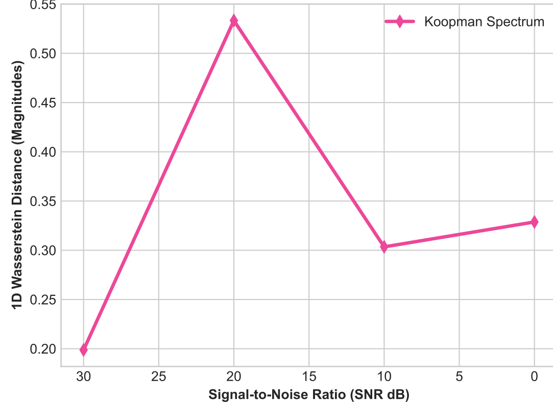
Koopman Operator Eigenvalue Stability
