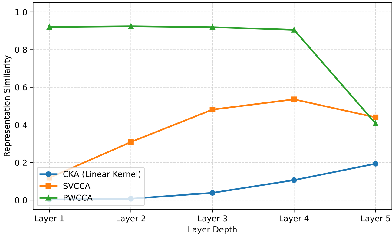
Representation Similarity under Domain Shift (SimpleLSTM1D)
