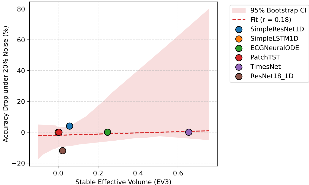
Representational Volume (EV3) vs Noise Sensitivity
