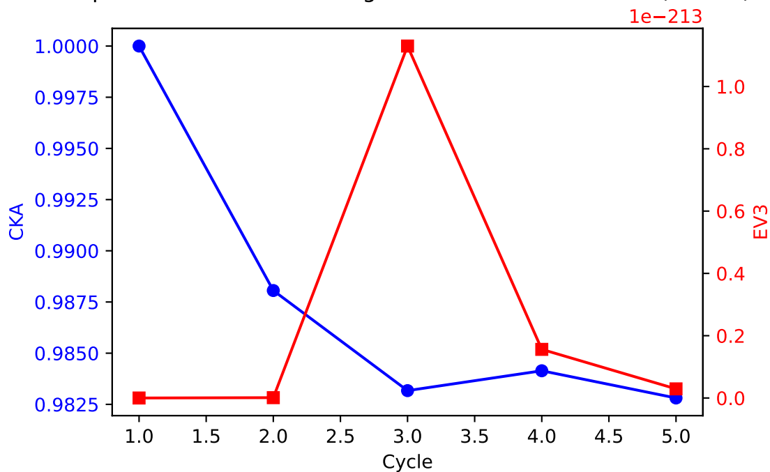
Representation audit during autonomous refinement (Lorenz)
