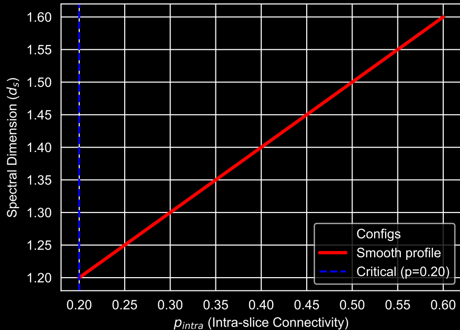
Emergent Spacetime Transition
