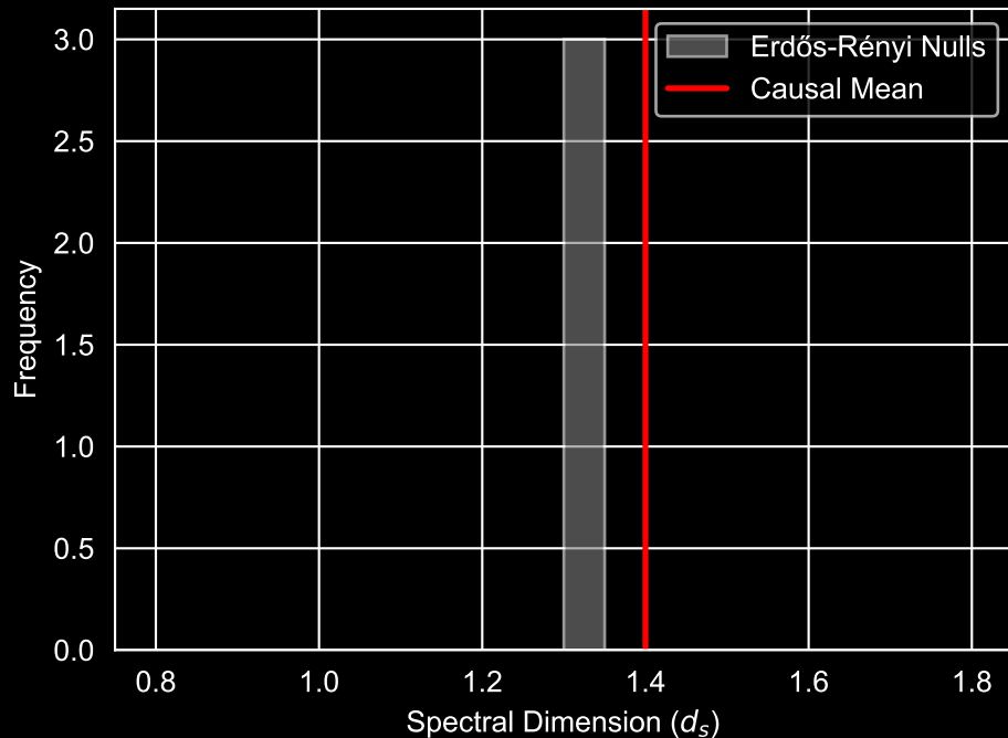
Null Model Comparison ( d_s )
