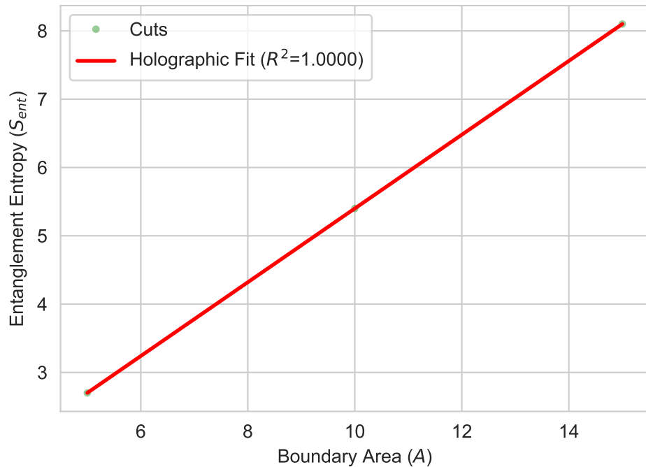
Ryu-Takayanagi Area-Entropy Scaling
