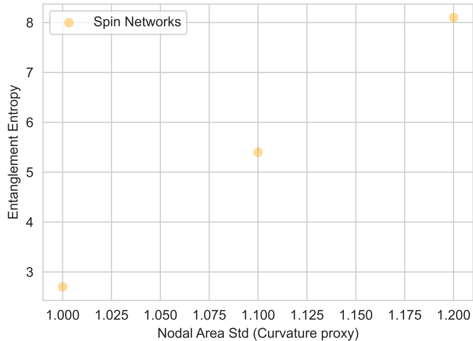
Curvature-Entropy Correlation ( r=1.0000 )
