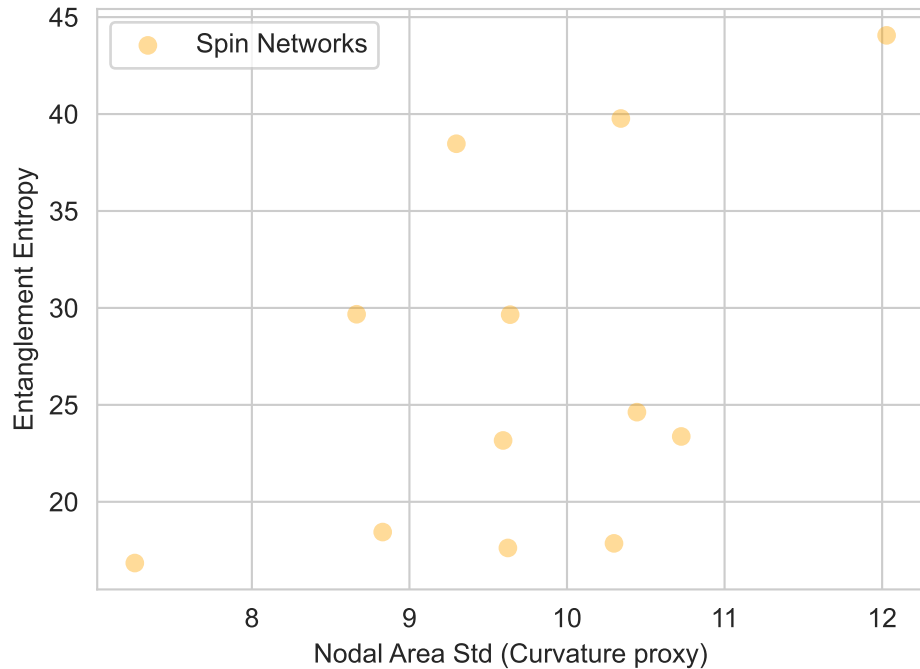
Curvature-Entropy Correlation ( r=0.5049 )
