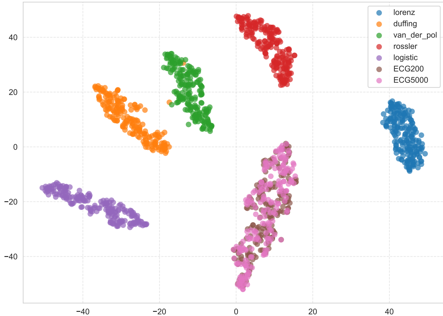
Dynamic Feature Space Projection (t-SNE)
