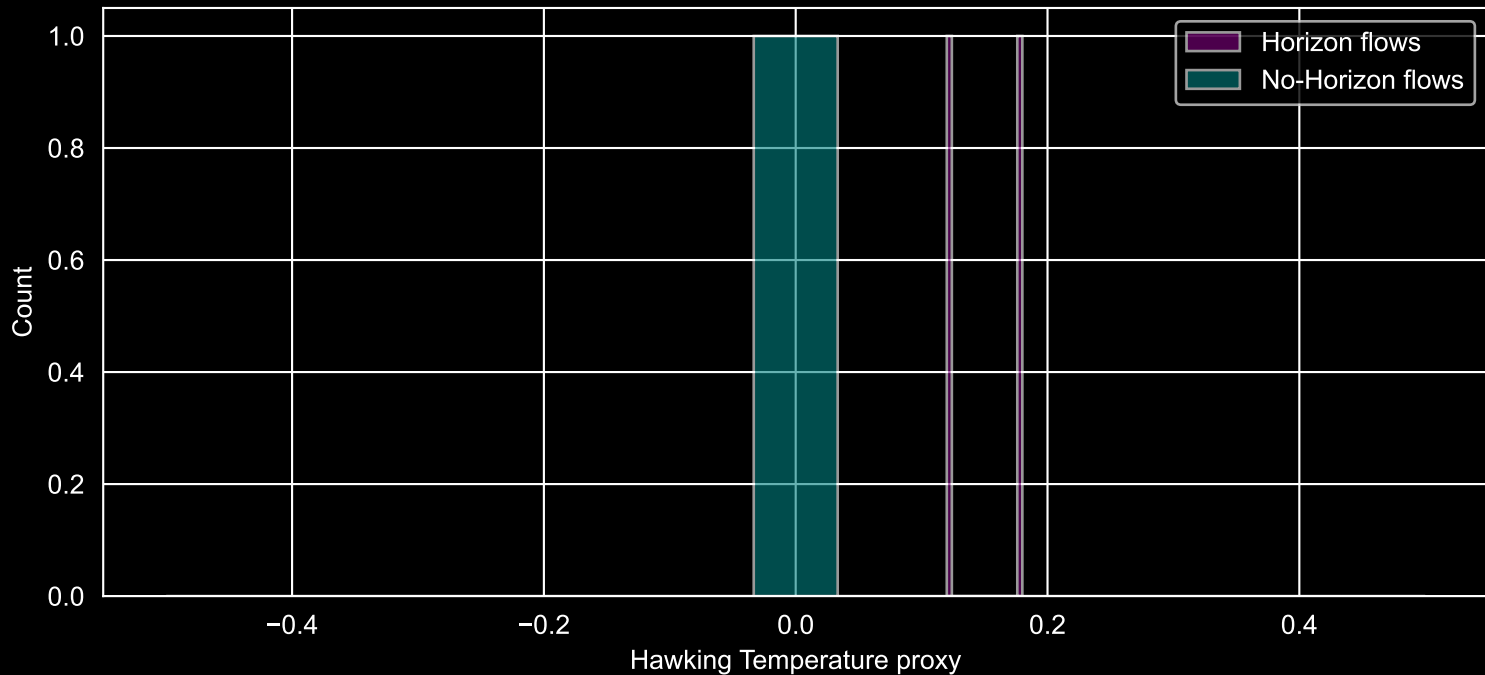
Horizon Topology Audit (Wasserstein d=0.1500)
