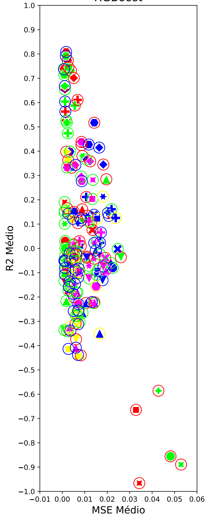
XGBoost
