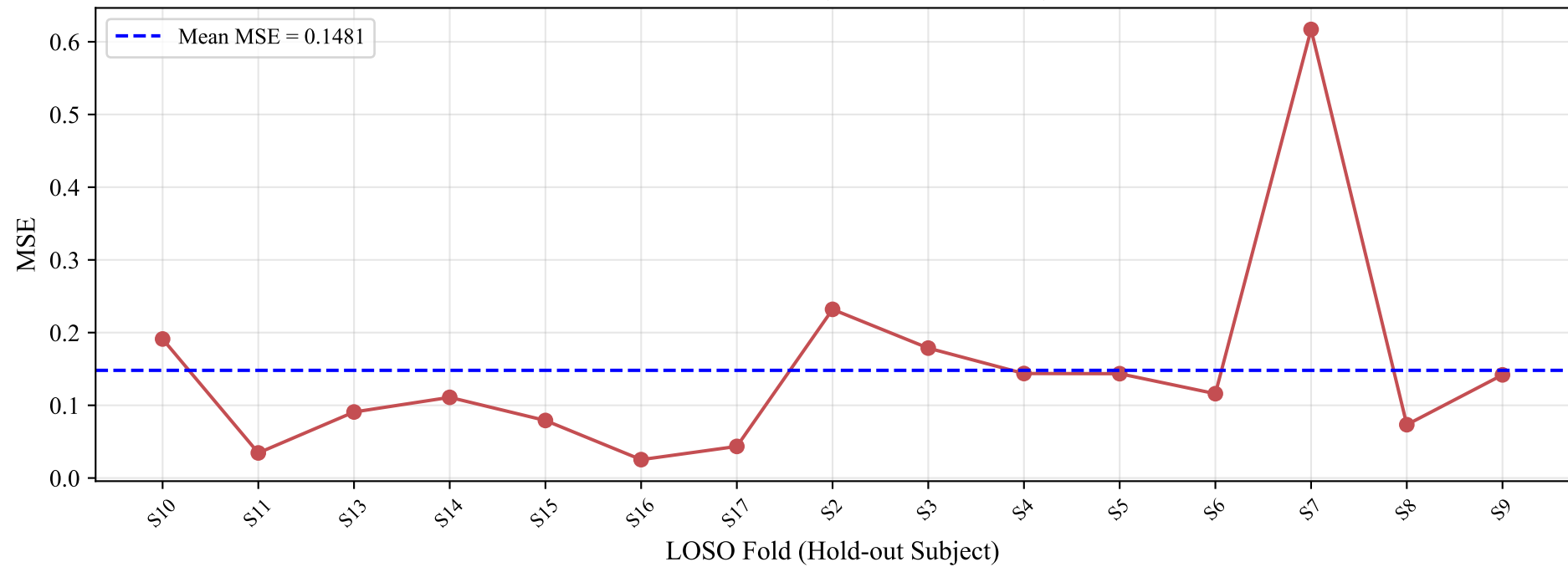
Per-fold Test MSE (Final Ours, 15 folds)
