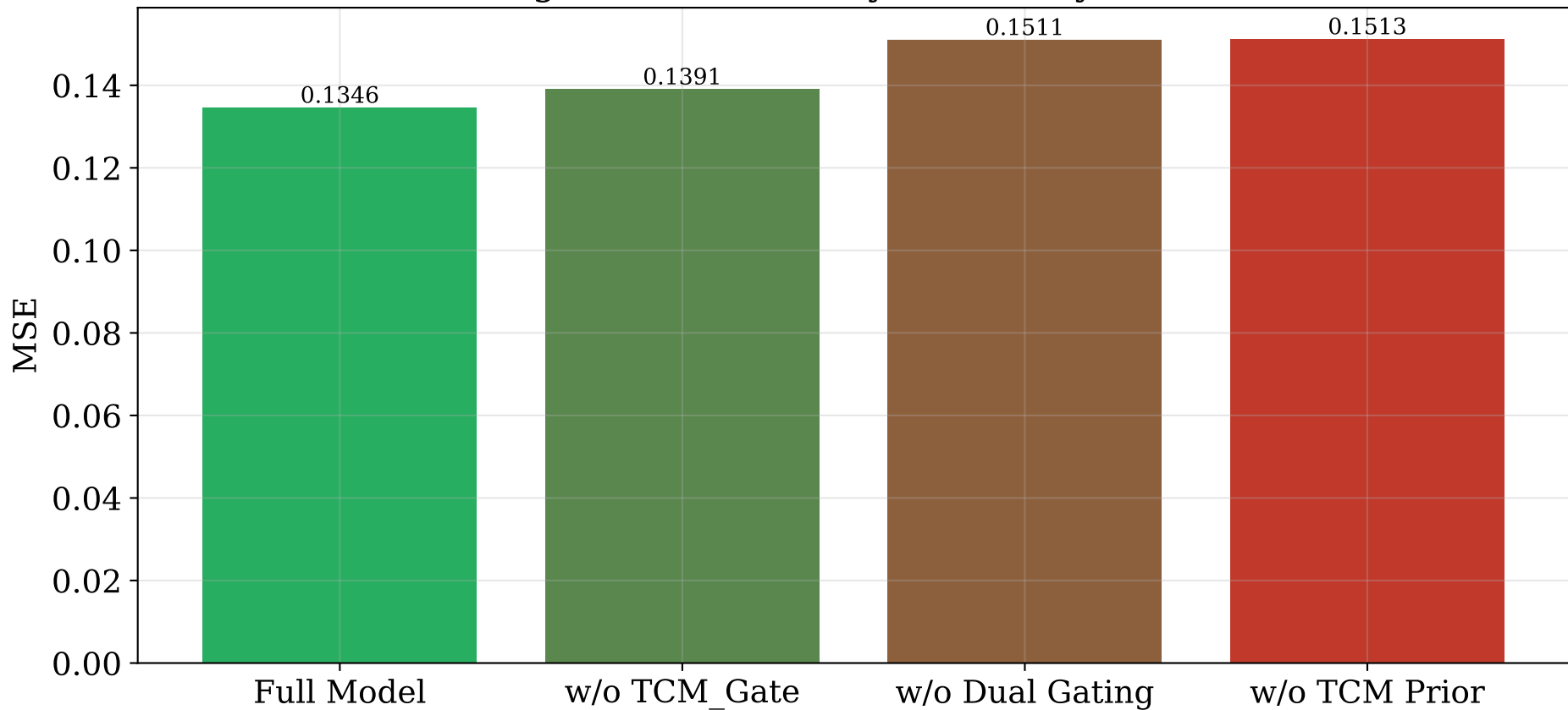
Fig.3 Ablation Study (sorted by MSE)
