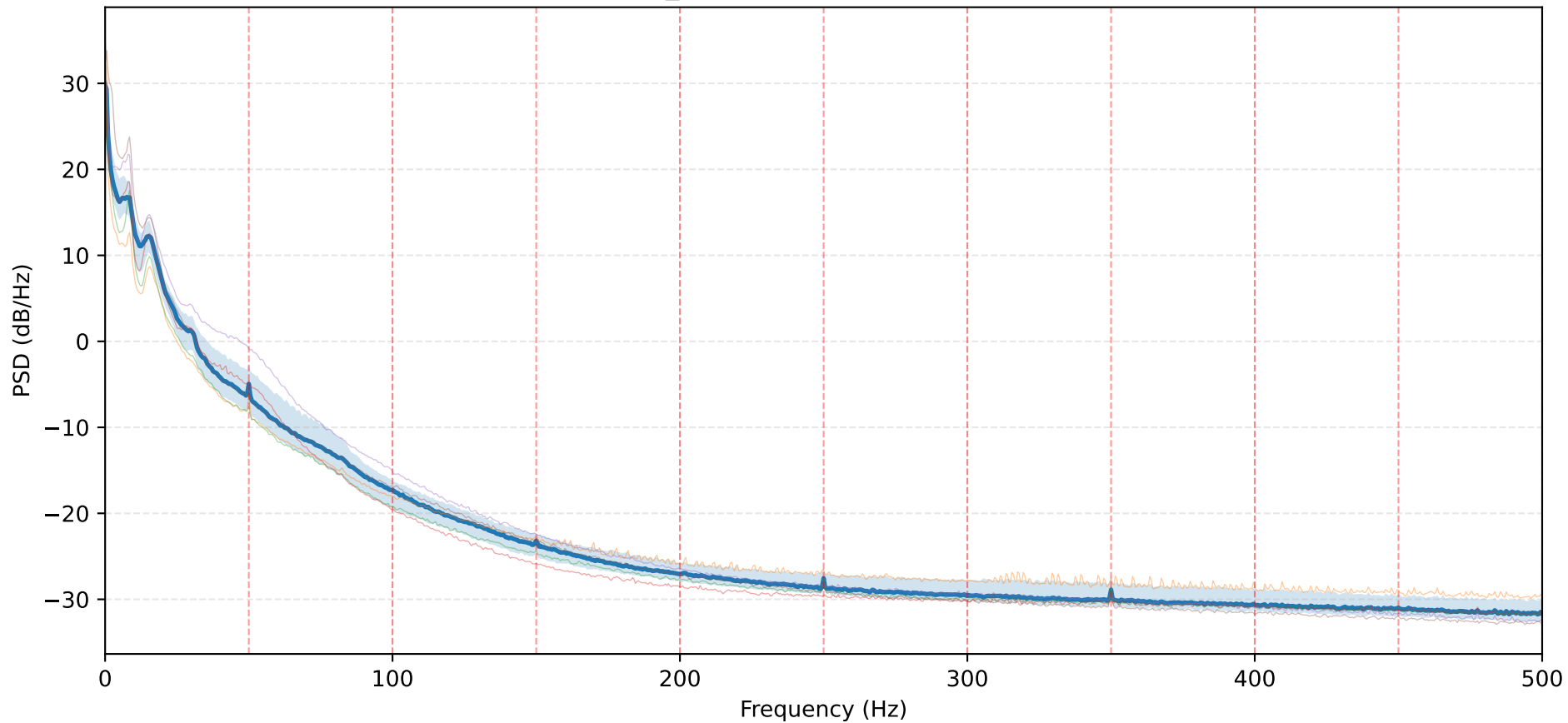
PAT_2868 - LM - PSD overview
