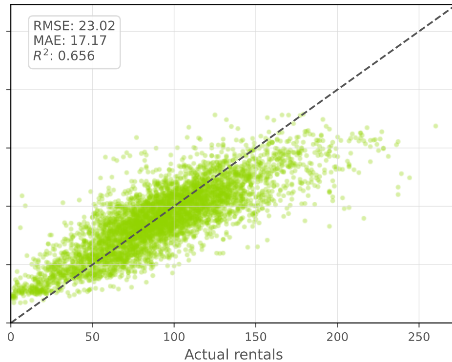
Random Forest
