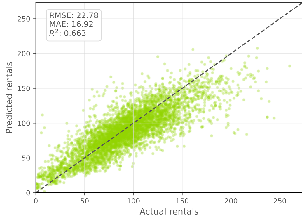
Gradient Boosting
