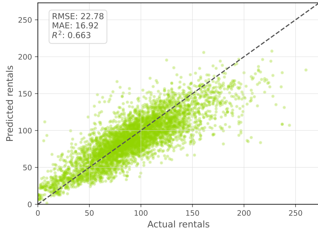
Gradient Boosting
