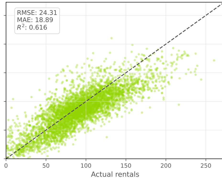
Neural Network
