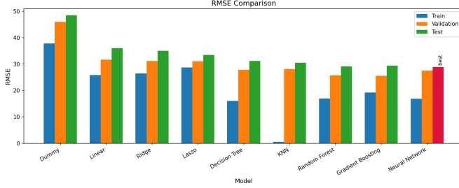
Fig. 2. Train, validation, and test RMSE across models. Large gaps between training and test RMSE indicate overfitting. KNN and the single Decision Tree show the clearest pattern, while ensemble methods generalize more reliably.
