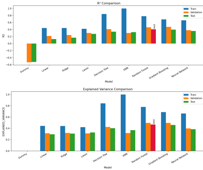
Fig. 3: R^2 and explained variance comparison. The same pattern appears in both views: the ensemble models explain the largest share of the target variation.
