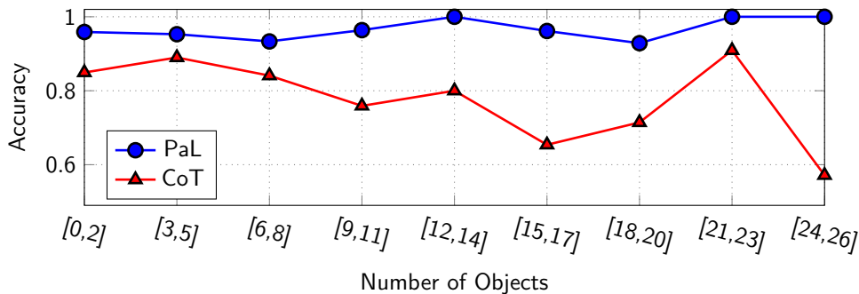
Figure: The solve rate on Colored Objects with respect to the number of objects included in the test question.
