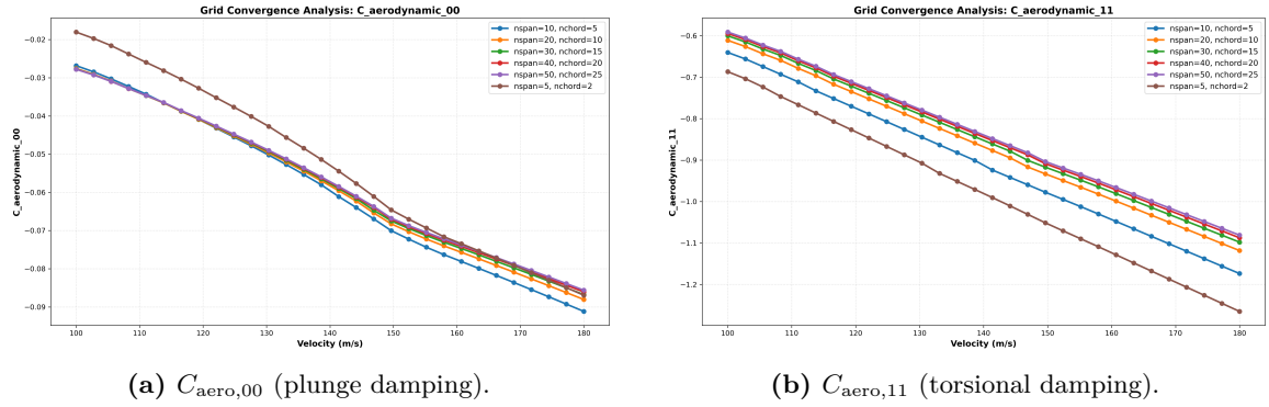
Figure 5.2: Aerodynamic damping matrix components (absolute values) as functions of velocity.
