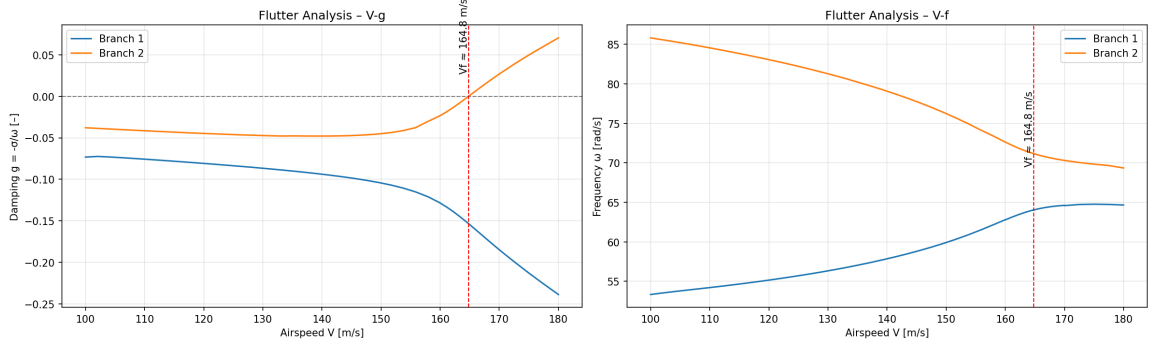
Figure 5.9: evaluated V-g and V-f diagrams for the Goland wing flutter analysis.
