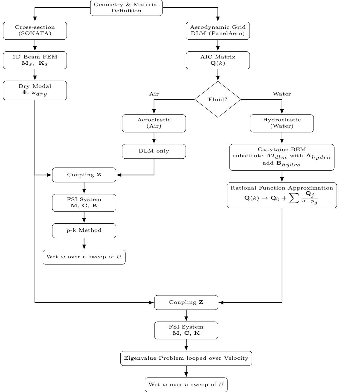
Figure 1.1: Unified workflow for aeroelastic and hydroelastic flutter analysis.
