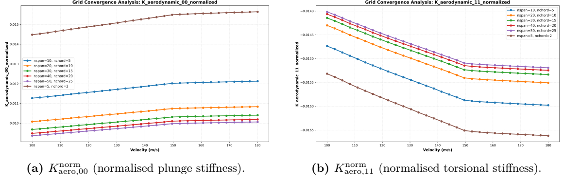
Figure 5.3: Normalised aerodynamic stiffness matrix components.
