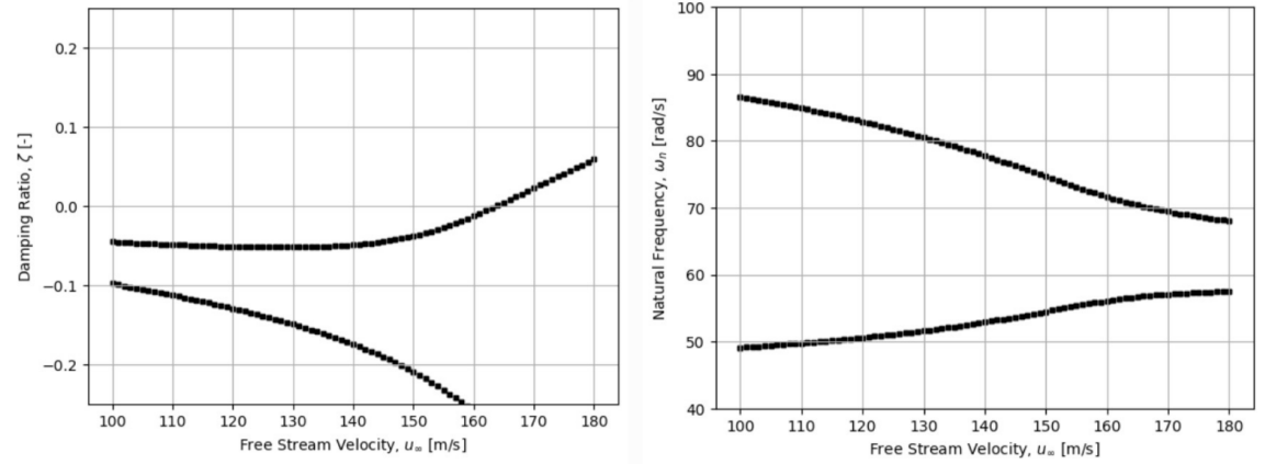
Figure 5.10: SHARPY V-g and V-f diagrams for the Goland wing flutter analysis.
