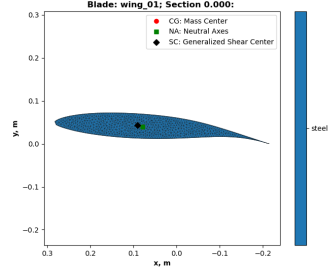
Figure 6.1: Cross-sectional view of the wing01.
