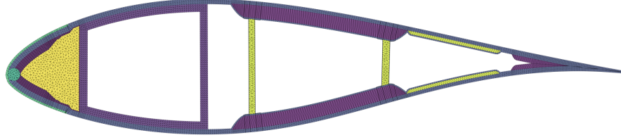
Figure 2.1: Example of a complex composite cross section handled by SONATA, representing the internal architecture of a 15-MW wind turbine blade. The figure is taken from [1].
