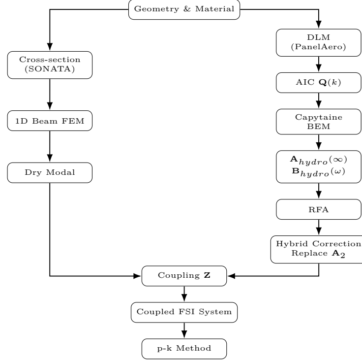
Figure 3.3: Hydroelastic analysis workflow: DLM combined with Capytaine BEM for rigorous water-based applications.
