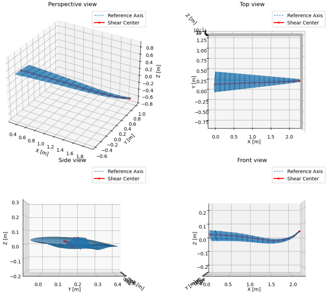
Figure 6.2: Detailed three-dimensional lofted surface geometry view of the wing01 modeled by SONATA.
