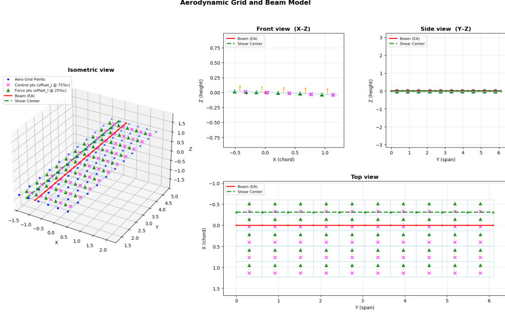
Figure 3.2: Aerodynamic grid and beam model showing the discretization and coupling schemes.
