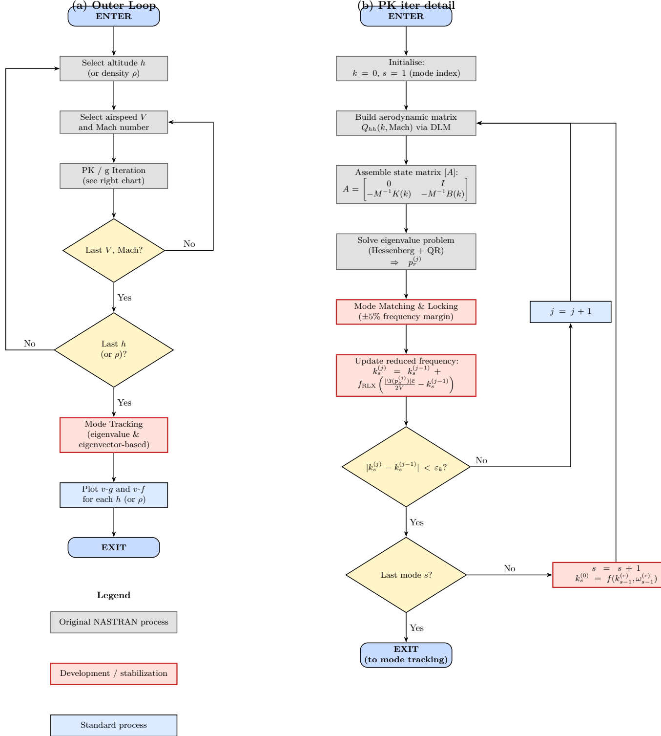
Figure 4.1: Schematic flowchart of the PK-method flutter analysis
