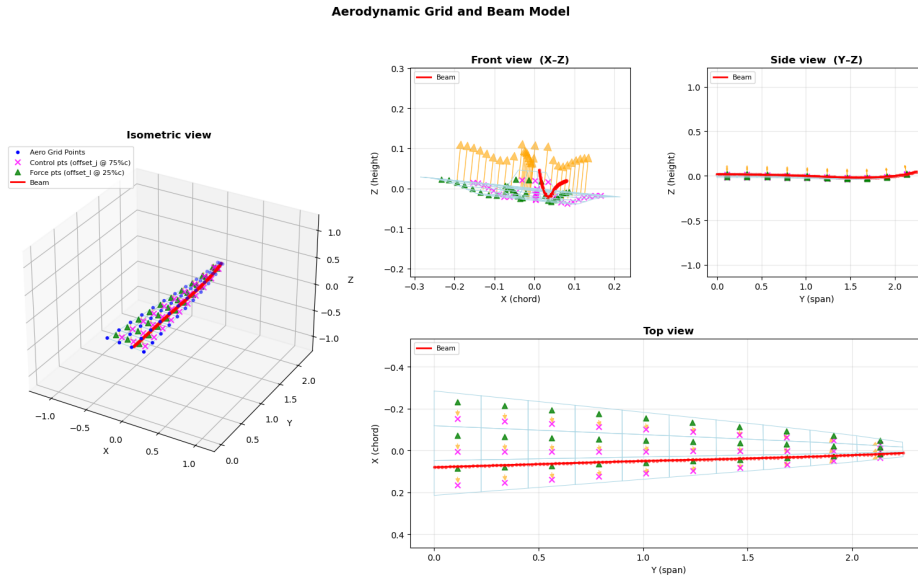
Figure 6.3: Three-dimensional views of the wing01 aero beam structure.
