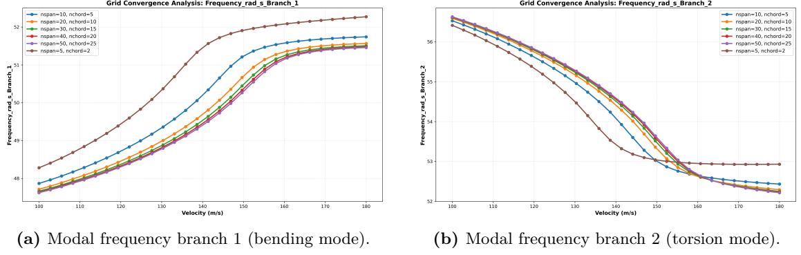
Figure 5.5: Structural modal frequencies in the velocity domain.
