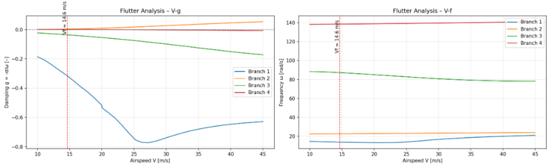
Figure 6.7: VG-VF flutter diagram for the tnz_multibody system. Results are modified to preserve confidentiality, but the general trends and critical flutter velocity are clearly indicated.
