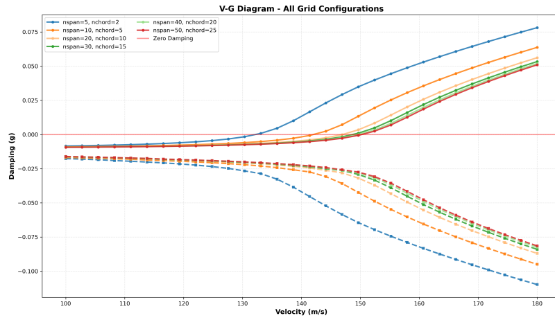
Figure 5.7: Combined V-G diagram for all grid configurations.
