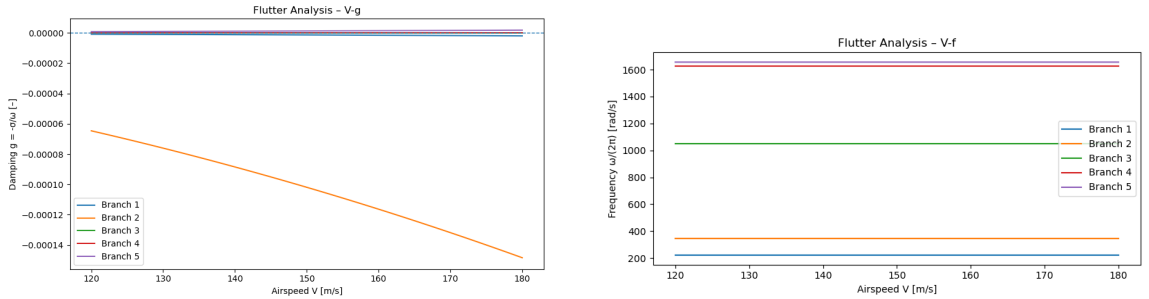
(a) Computed vg trajectories for the wing01 case.
