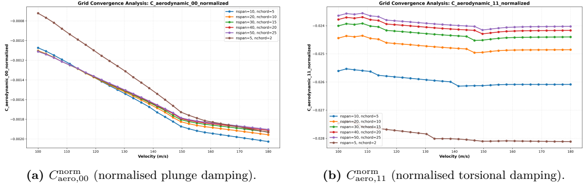
Figure 5.4: Normalised aerodynamic damping matrix components.
