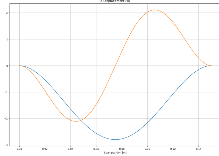
Figure 5.13: NACA0003 dry mode shapes for the first and second mode.
