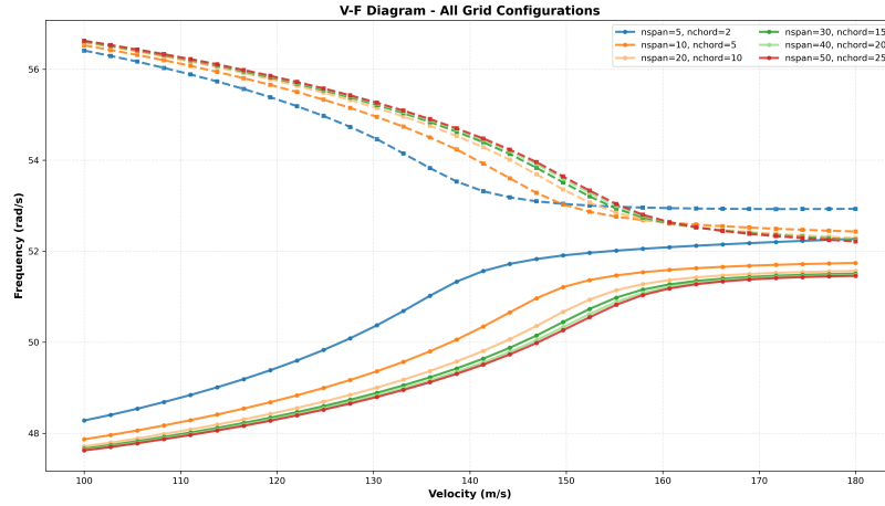
Figure 5.6: Combined V-F diagram for all grid configurations.
