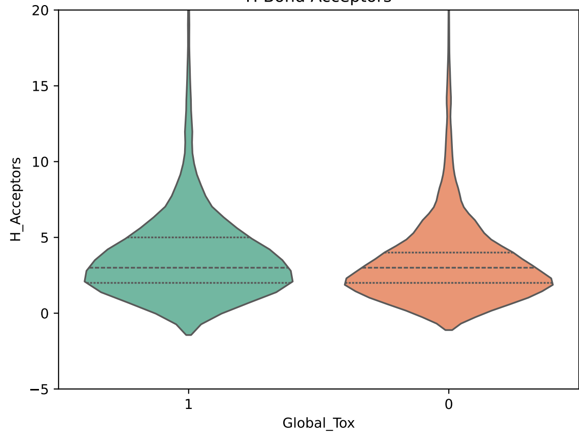
H-Bond Acceptors
