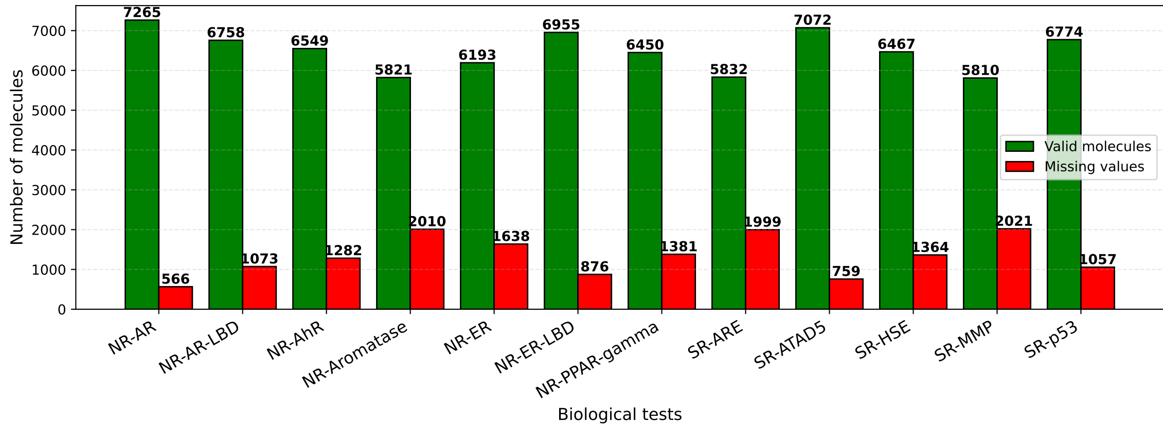
TOX21: Valid vs Missing tests
