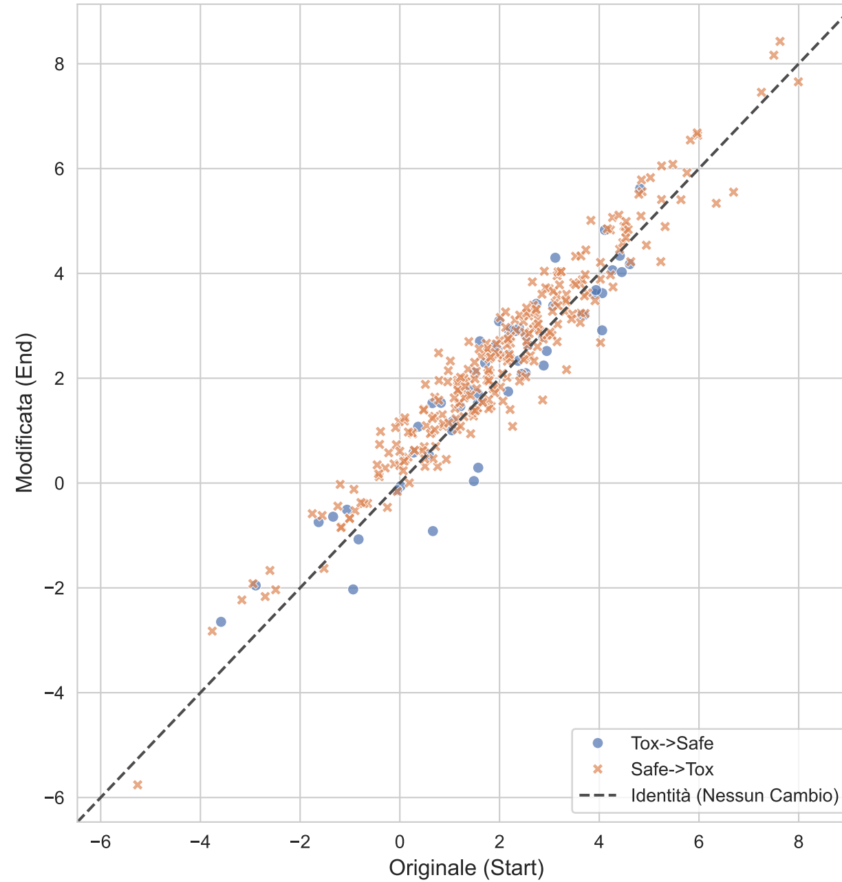
LogP (Lipophilicity) Preservation
