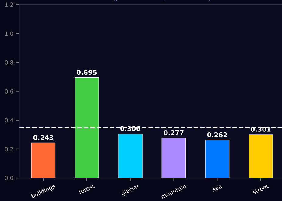
Average Precision (mAP=0.347)
