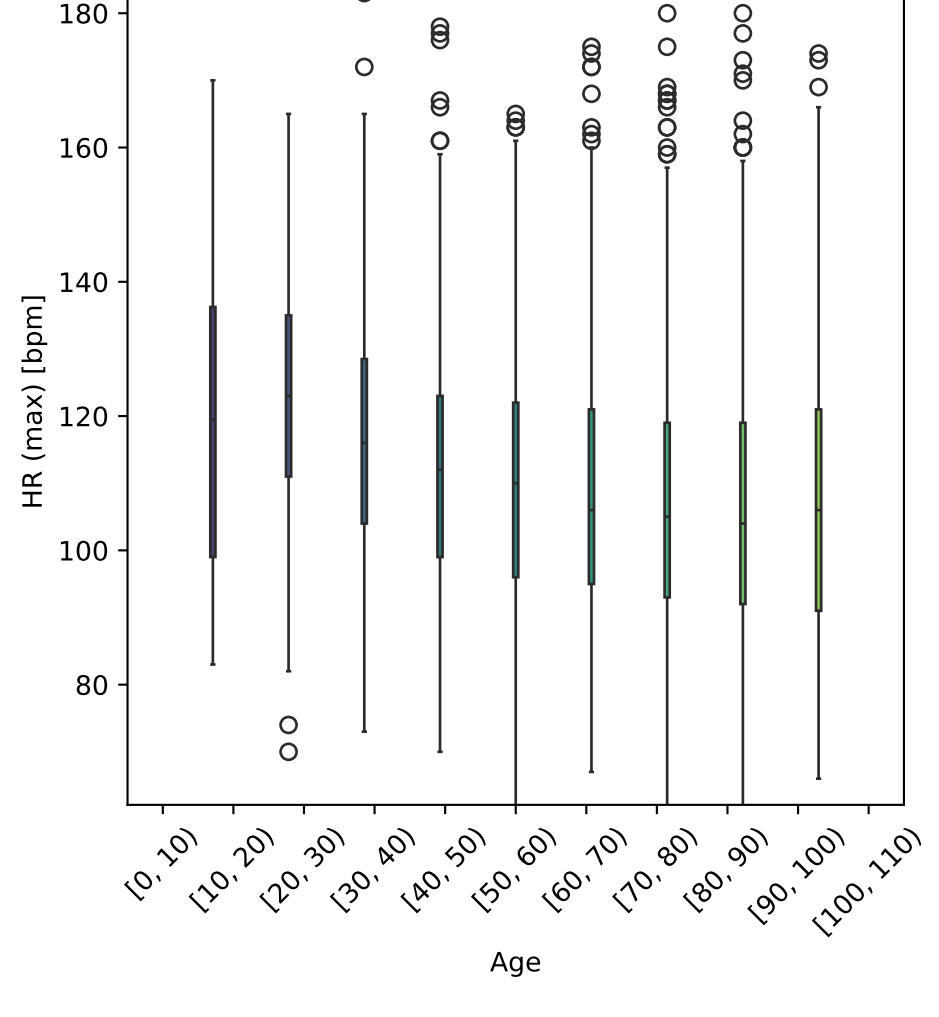
HR (max) vs Age Tot. num. of data points: 2937
