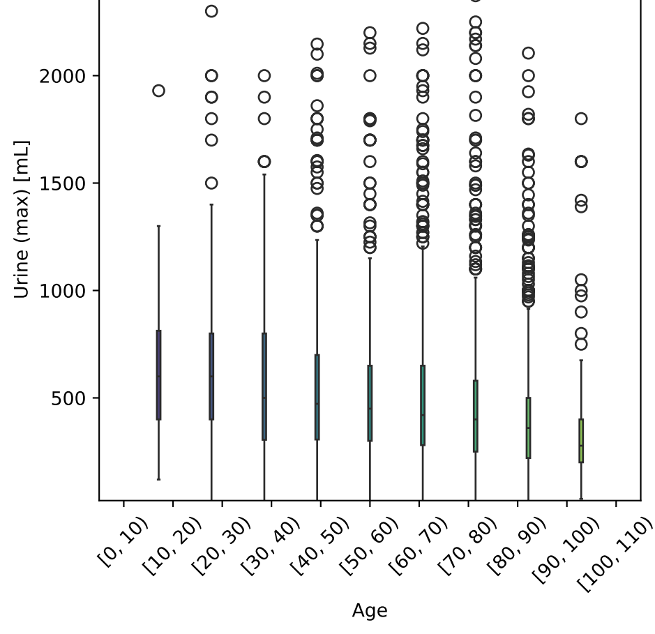
Urine (max) vs Age Tot. num. of data points: 2493
