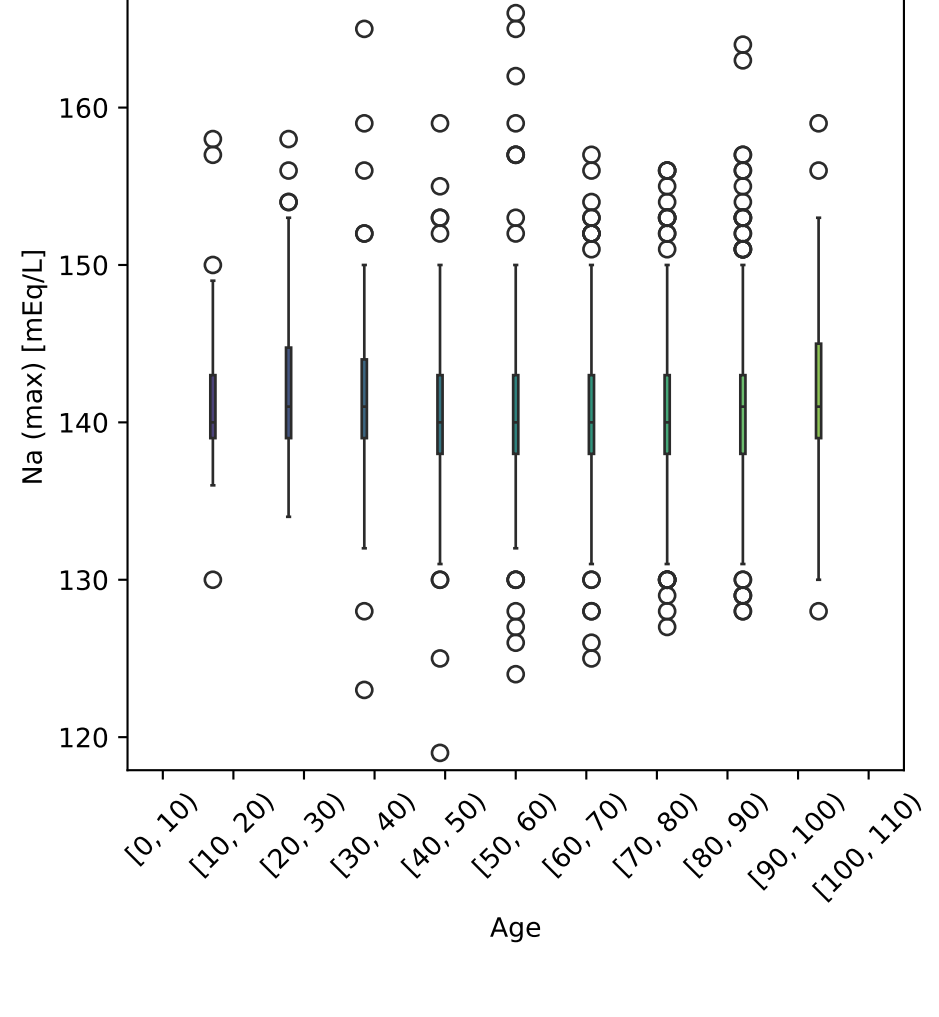
Na (max) vs Age Tot. num. of data points: 2925
