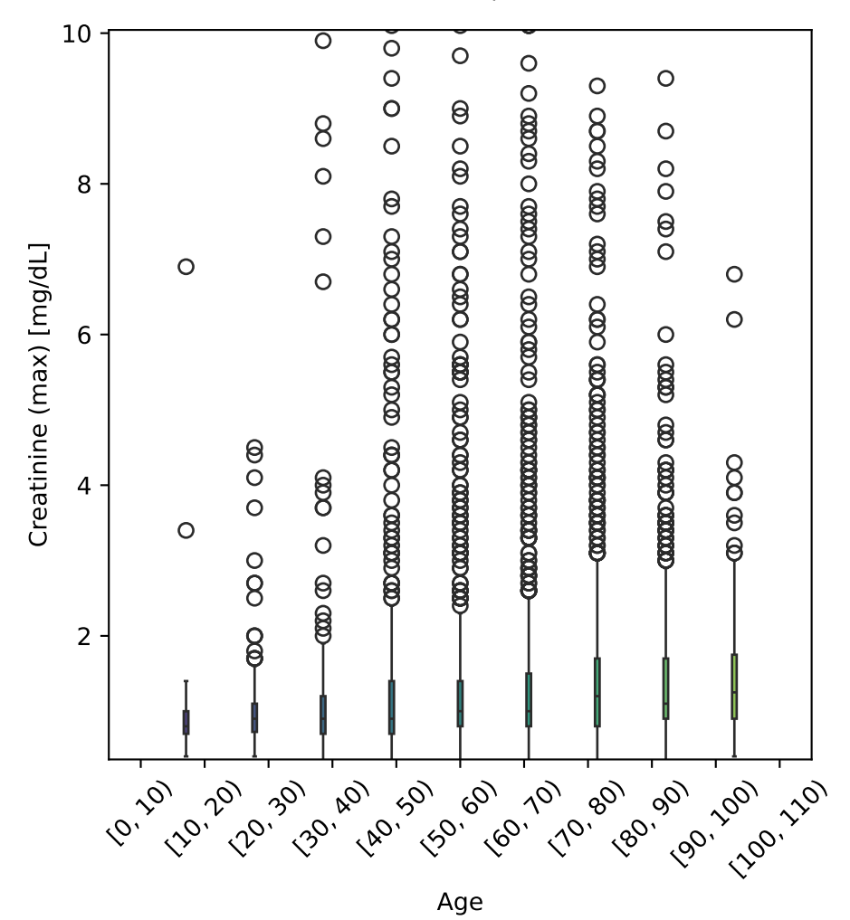
Creatinine (max) vs Age Tot. num. of data points: 3934
