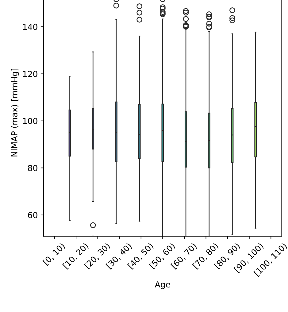
NIMAP (max) vs Age Tot. num. of data points: 2821
