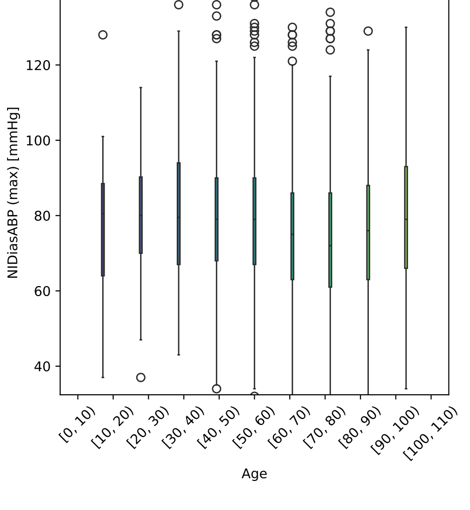
NIDiasABP (max) vs Age Tot. num. of data points: 3493
