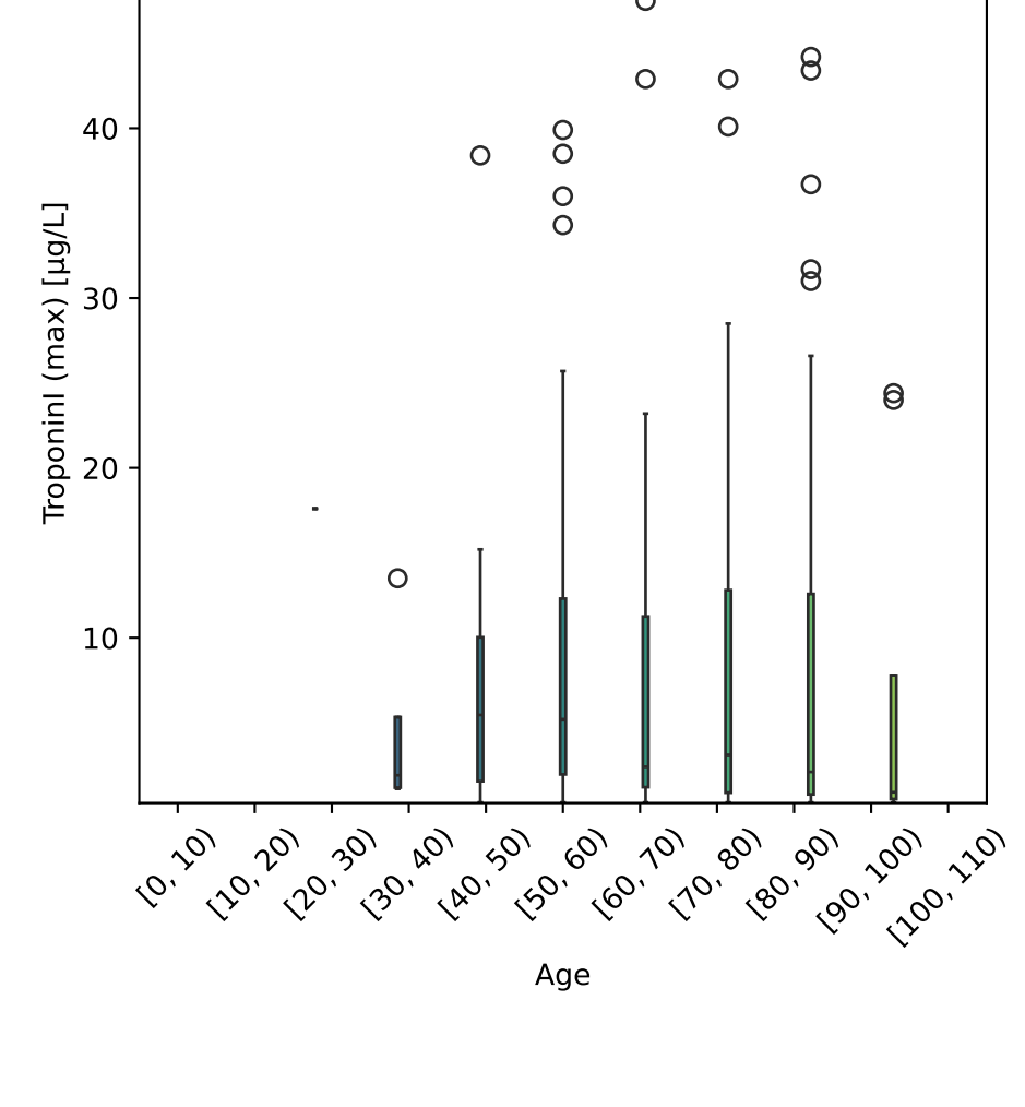
TroponinI (max) vs Age Tot. num. of data points: 209
