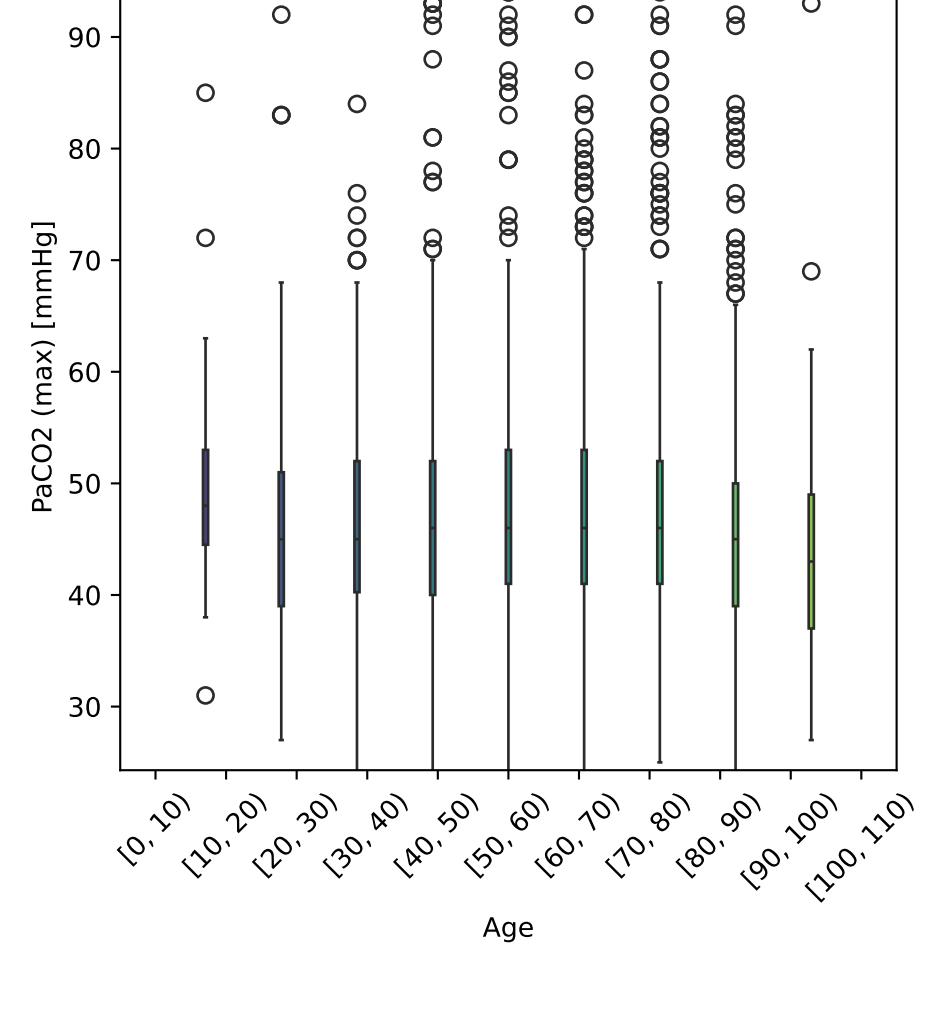
PaCO2 (max) vs Age Tot. num. of data points: 3623
