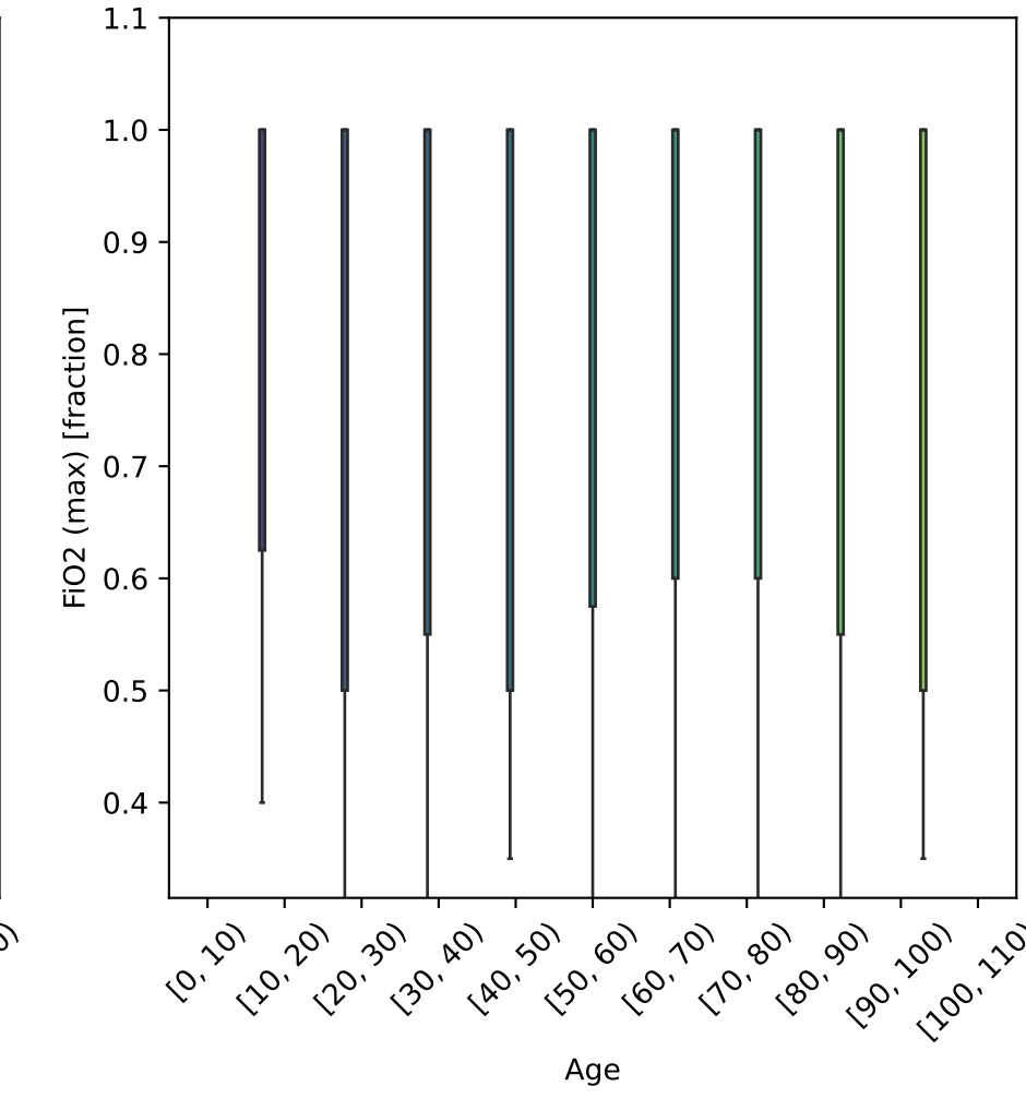
FI02 (max) vs Age Tot. num. of data points: 2717
