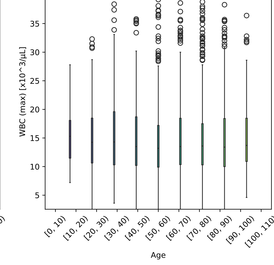
WBC (max) vs Age Tot. num. of data points: 2927
