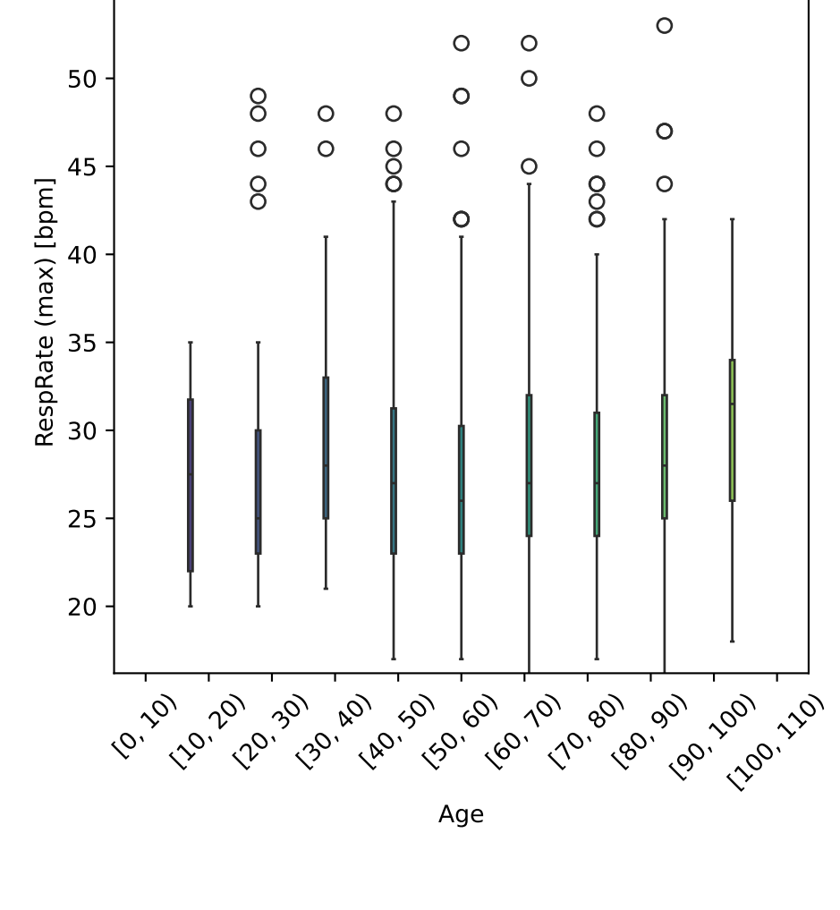
RespRate (max) vs Age Tot. num. of data points: 1192
