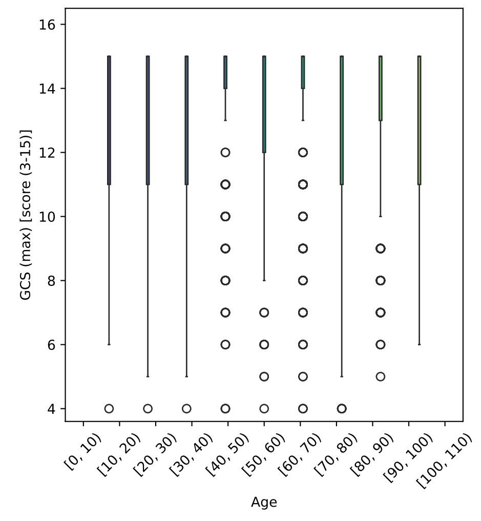
GCS (max) vs Age Tot. num. of data points: 2936
