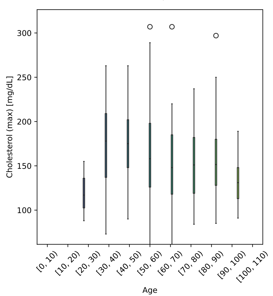
Cholesterol (max) vs Age Tot. num. of data points: 309
