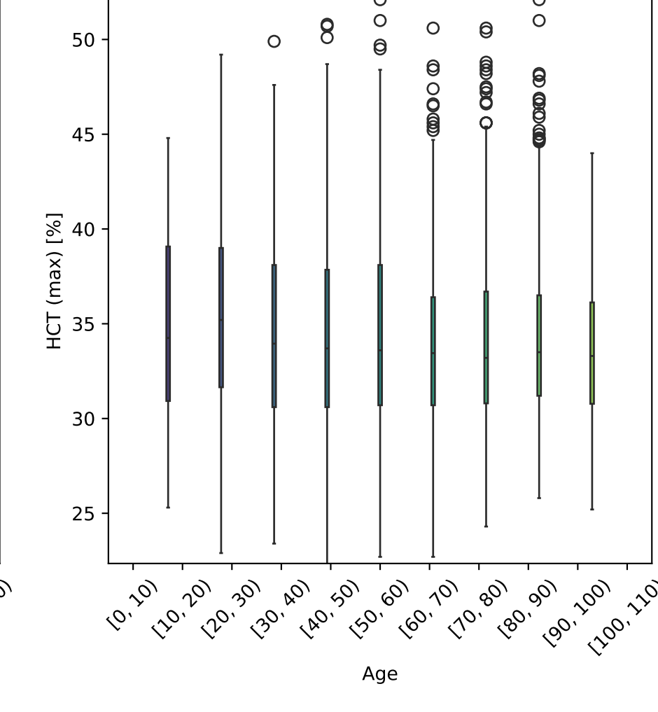
HCT (max) vs Age Tot. num. of data points: 2936
