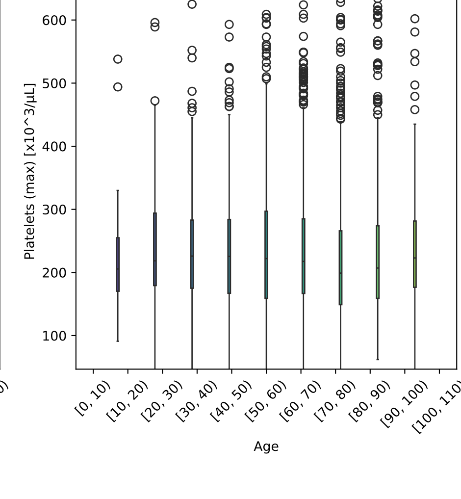
Platelets (max) vs Age Tot. num. of data points: 2492
