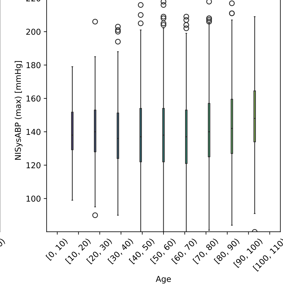
NISysABP (max) vs Age Tot. num. of data points: 2495
