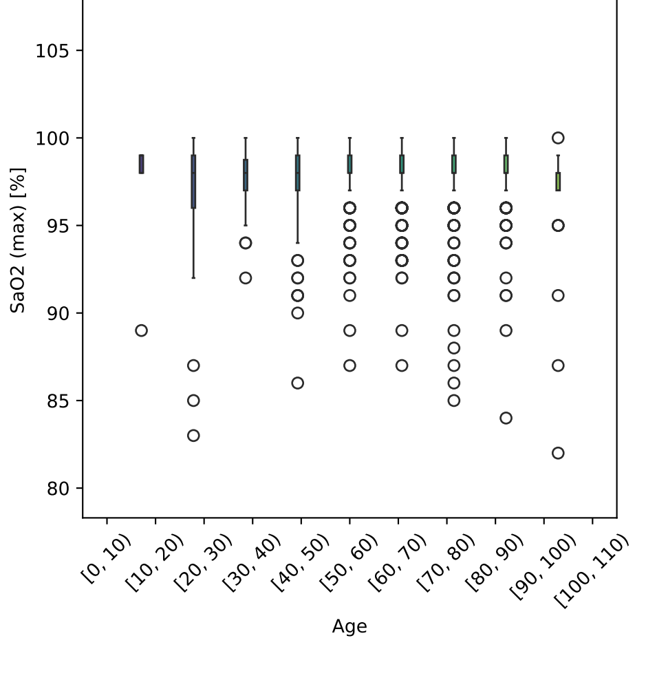
SaO2 (max) vs Age Tot. num. of data points: 2792
