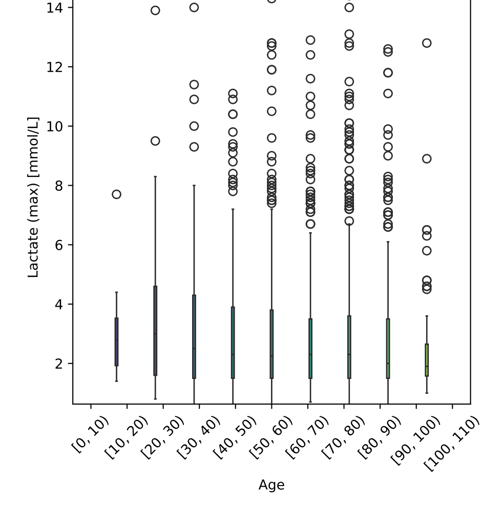
Lactate (max) vs Age Tot. num. of data points: 285
