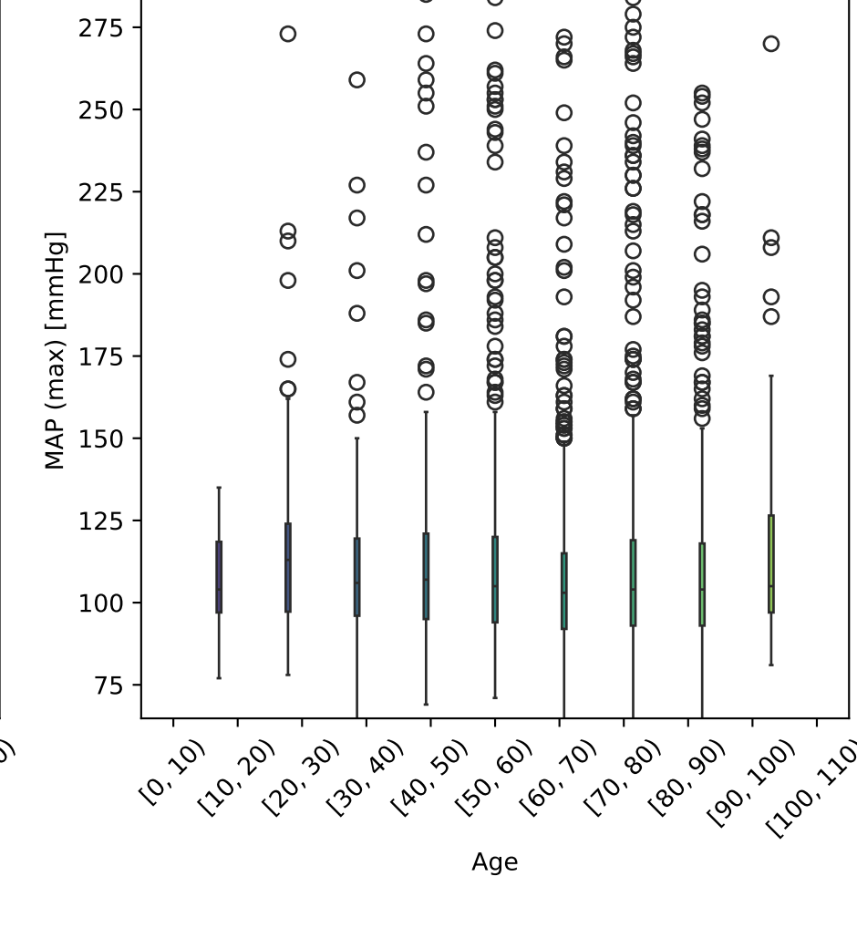
MAP (max) vs Age Tot. num. of data points: 2792
