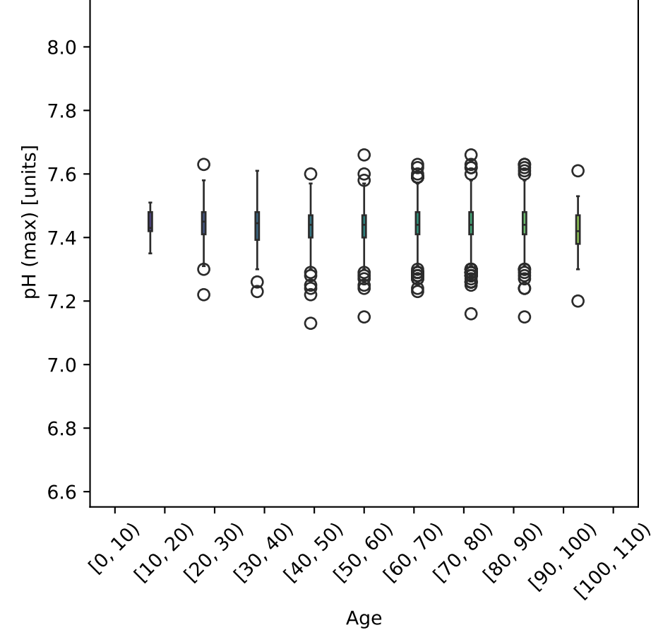
pH (max) vs Age Tot. num. of data points: 2040
