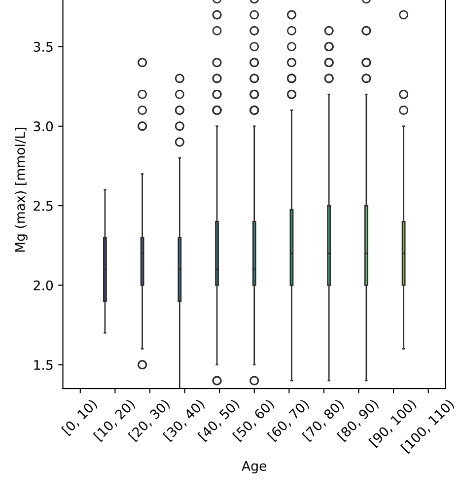
Mg (max) vs Age Tot. num. of data points: 2897
