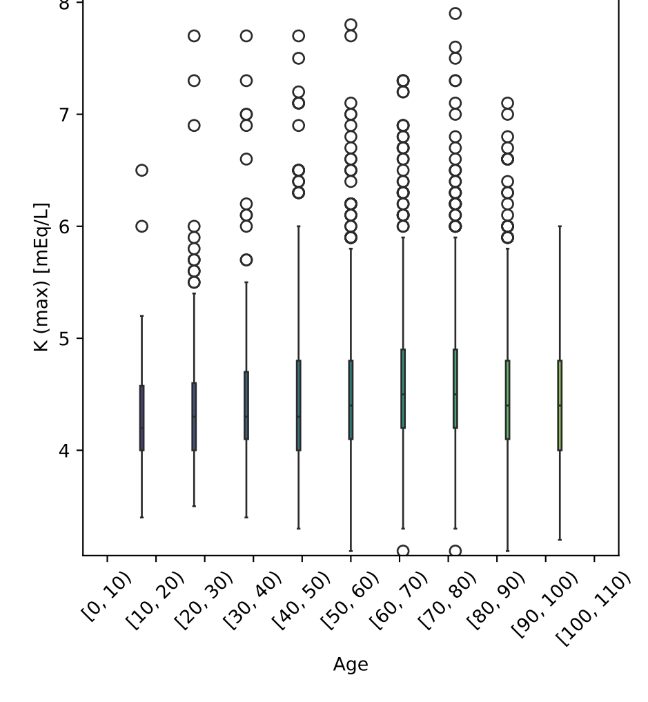
K (max) vs Age Tot. num. of data points: 3904
