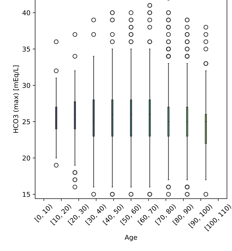
HCO3 (max) vs Age Tot. num. of data points: 2924
