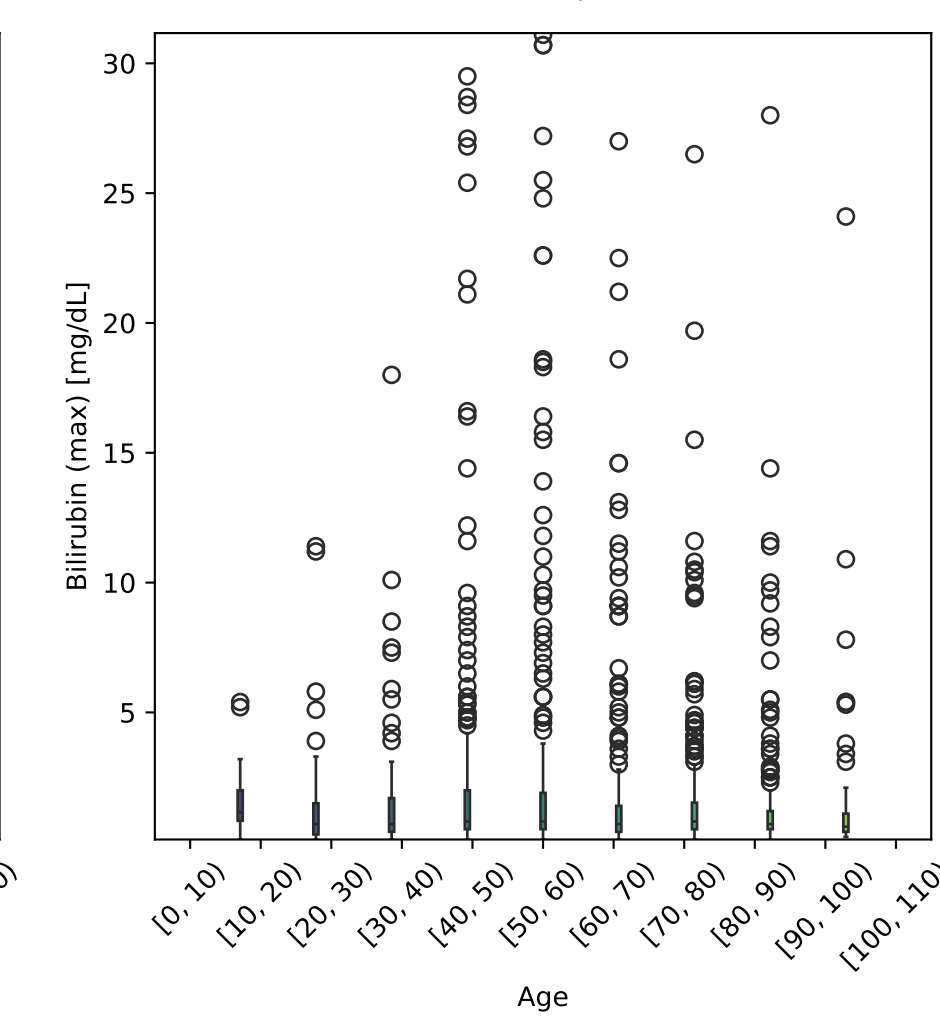
Bilirubin (max) vs Age Tot. num. of data points: 1748
