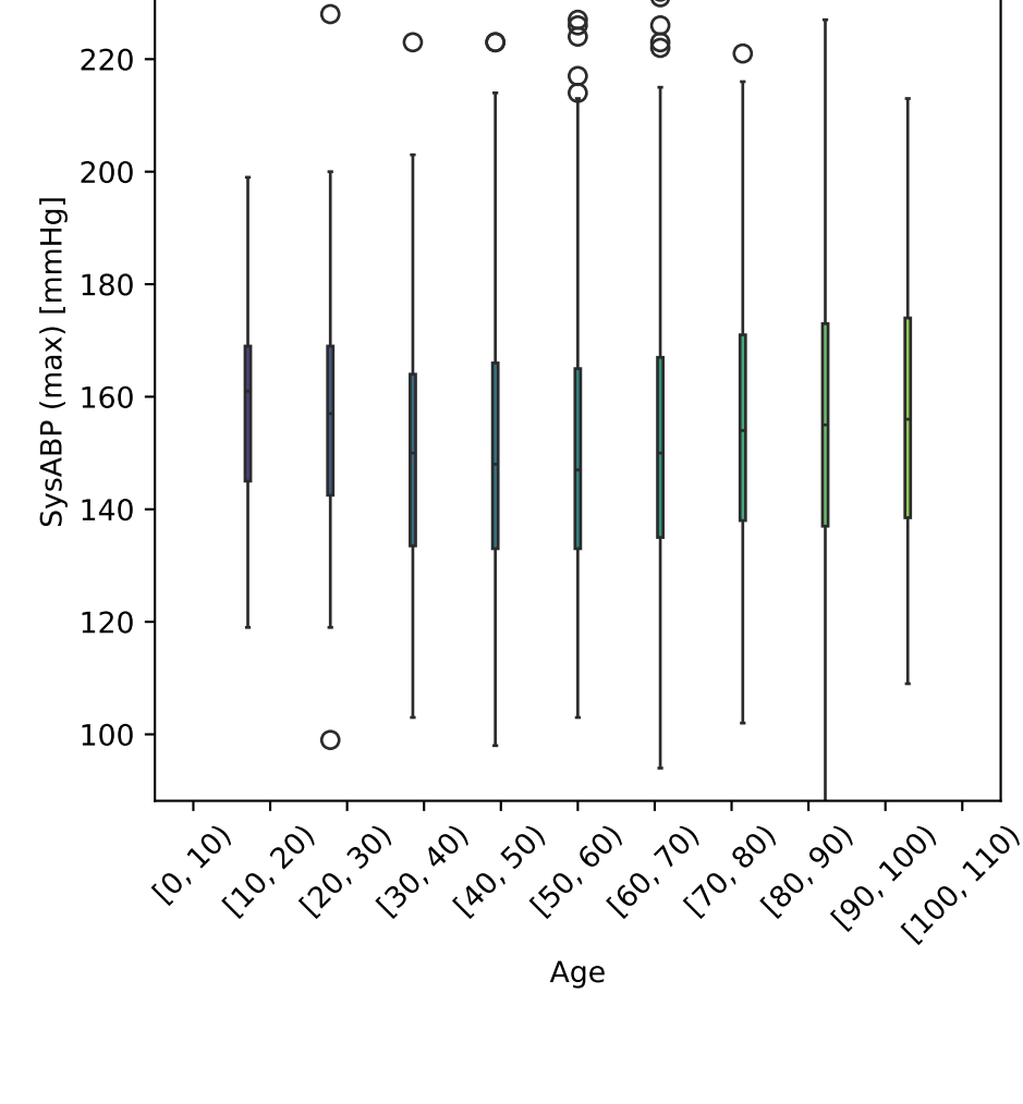
SysABP (max) vs Age Tot. num. of data points: 2495
