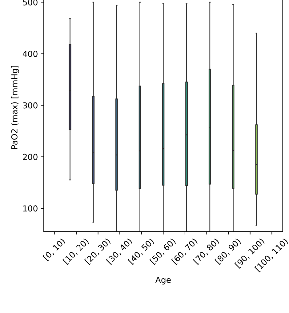
PaO2 (max) vs Age Tot. num. of data points: 3023
