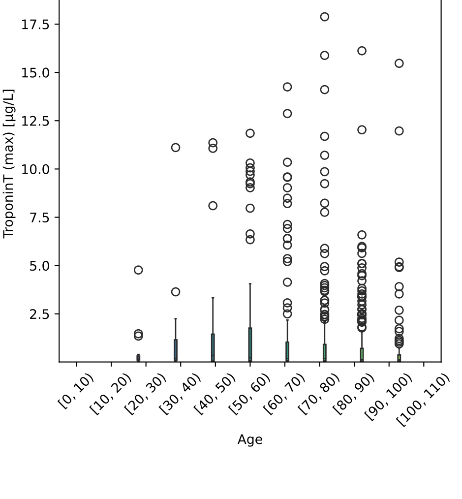
TroponinT (max) vs Age Tot. num. of data points: 699
