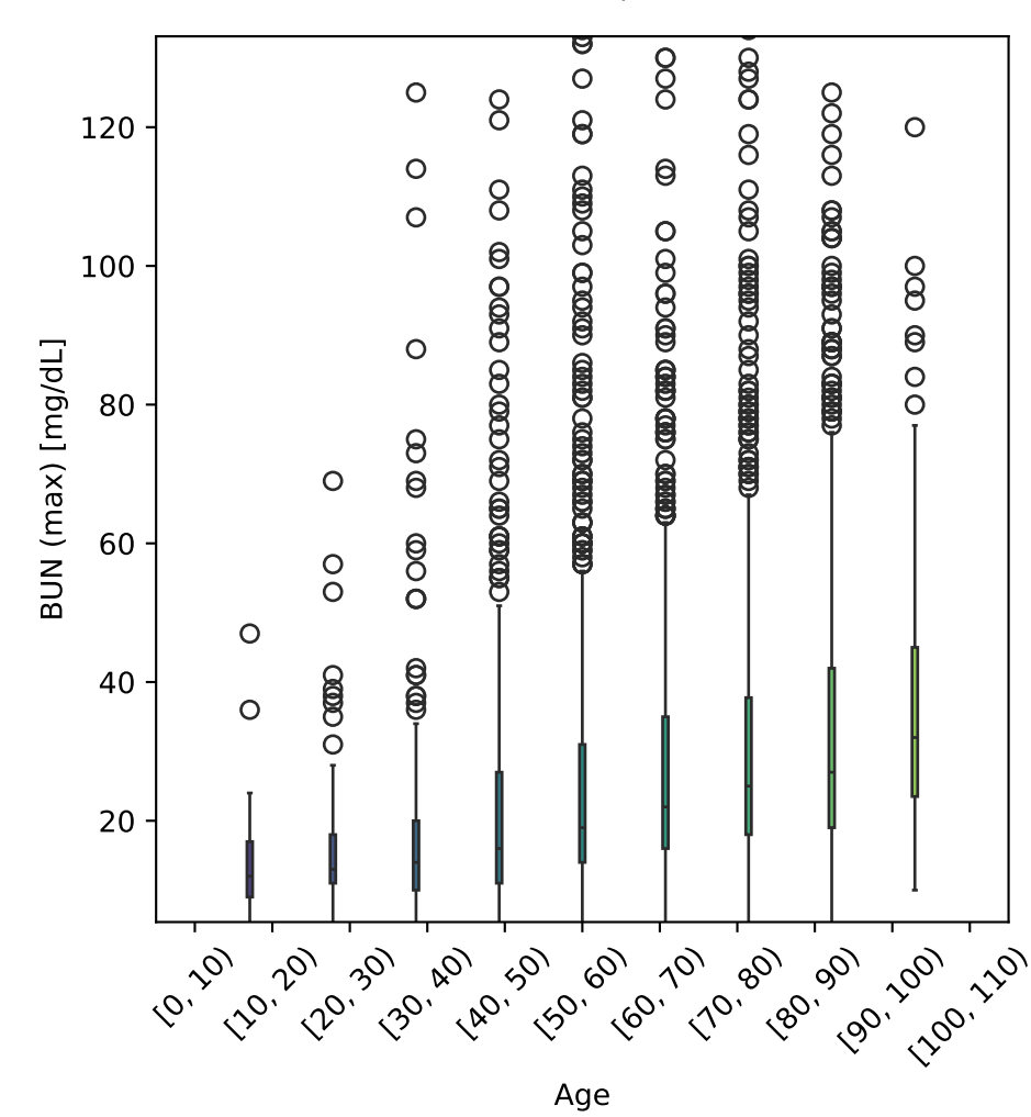
BUN (max) vs Age Tot. num. of data points: 2936
