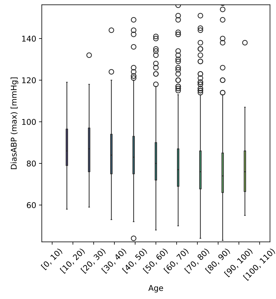
DiasABP (max) vs Age Tot. num. of data points: 2199
