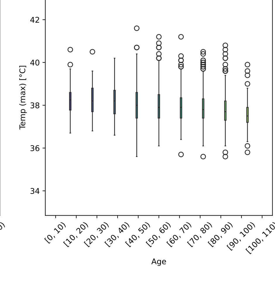
Temp (max) vs Age Tot. num. of data points: 2936
