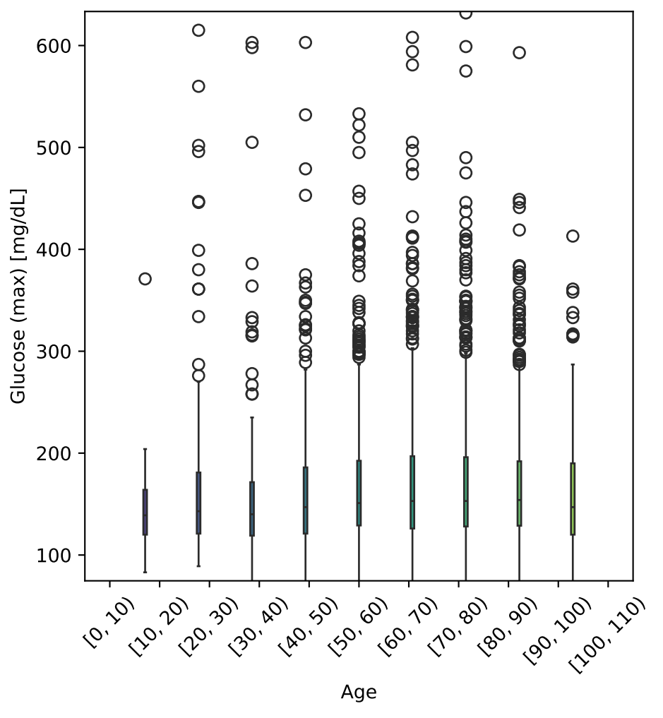
Glucose (max) vs Age Tot. num. of data points: 3947
