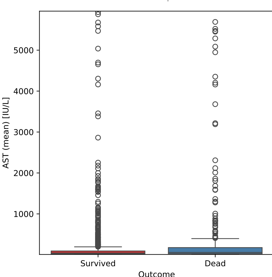
AST (mean) vs Outcome
