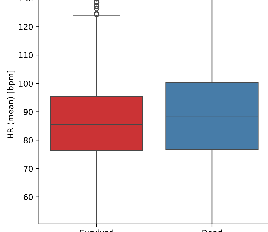
HR (mean) vs Outcome
