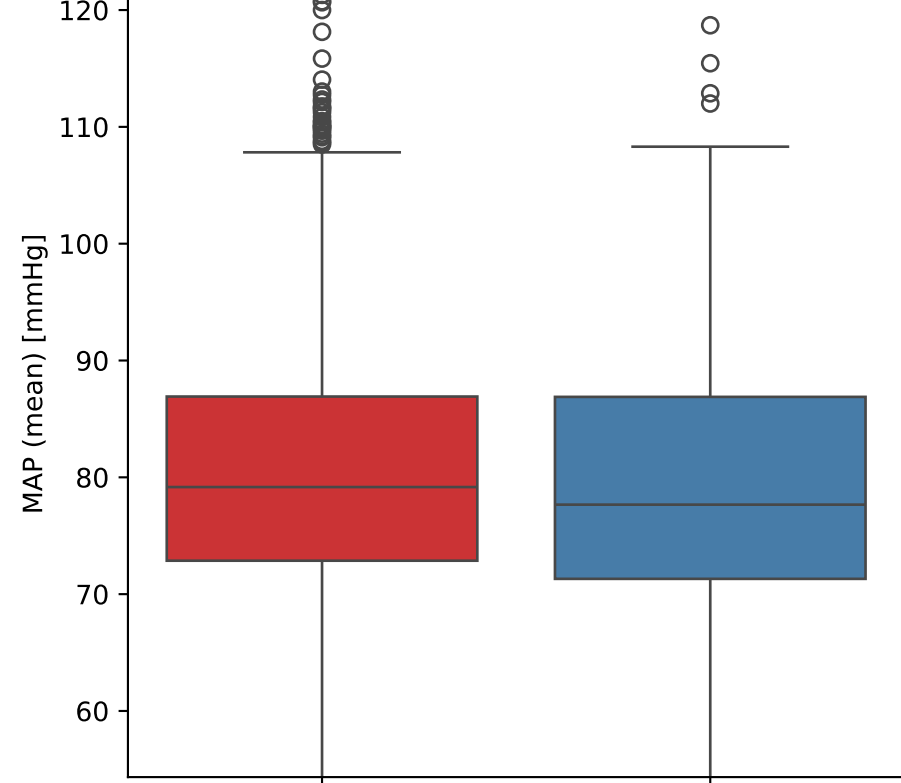
MAP (mean) vs Outcome
