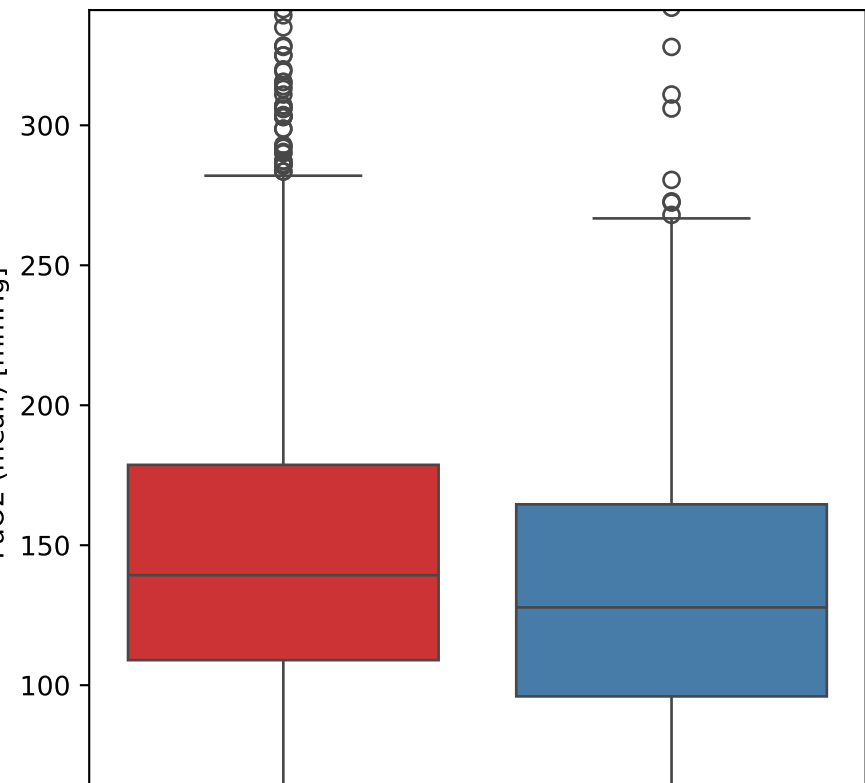
PaO2 (mean) vs Outcome
