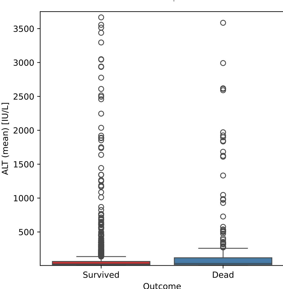
ALT (mean) vs Outcome
