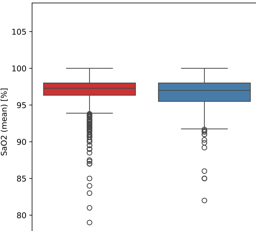
SaO2 (mean) vs Outcome
