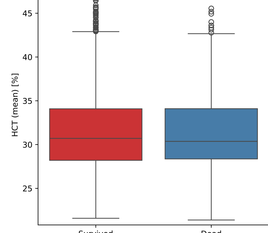
HCT (mean) vs Outcome
