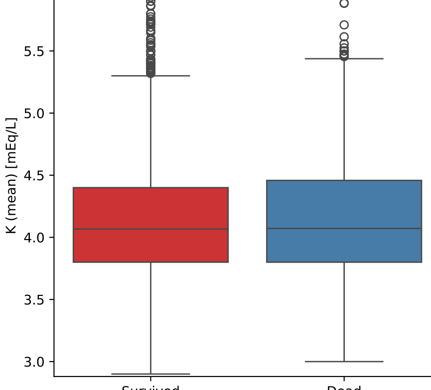
K (mean) vs Outcome
