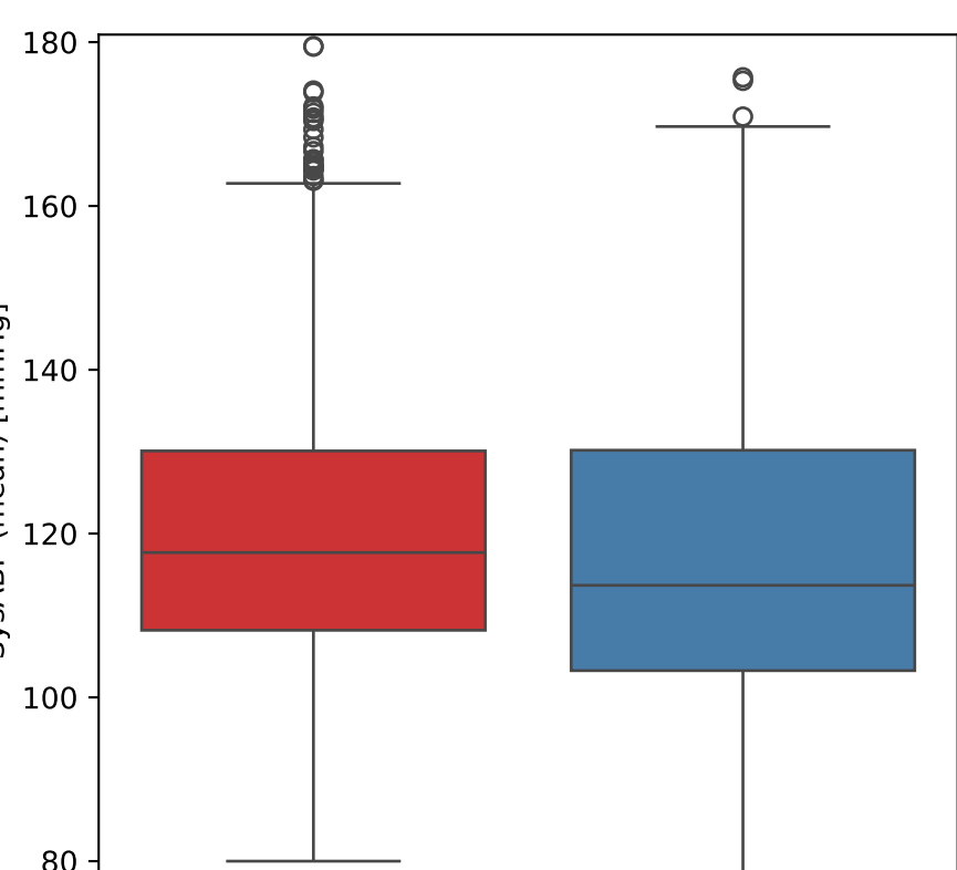
SysABP (mean) vs Outcome
