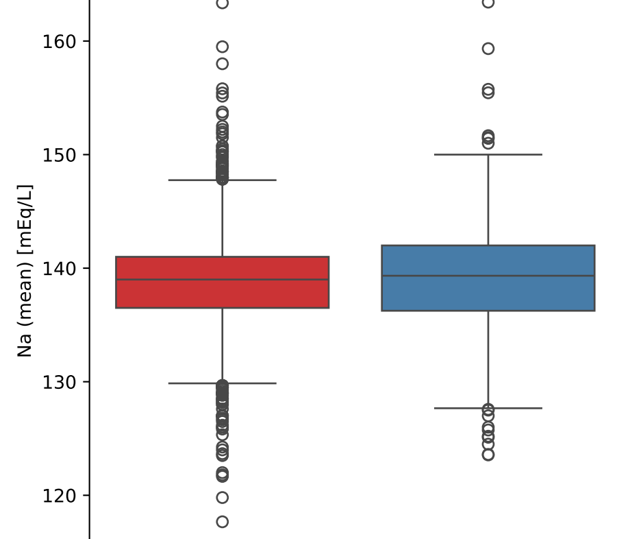
Na (mean) vs Outcome
