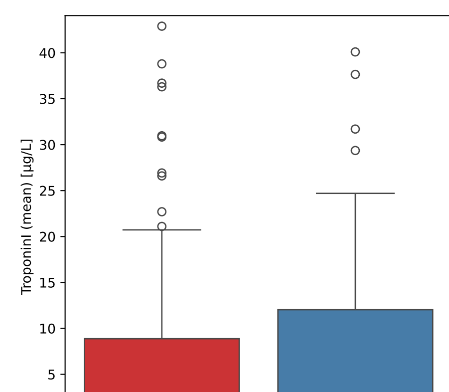
TroponinI (mean) vs Outcome
