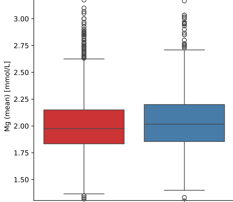
Mg (mean) vs Outcome
