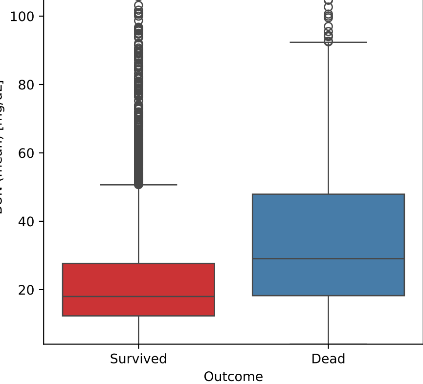
BUN (mean) vs Outcome
