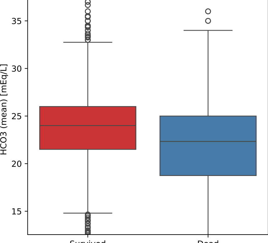
HCO3 (mean) vs Outcome
