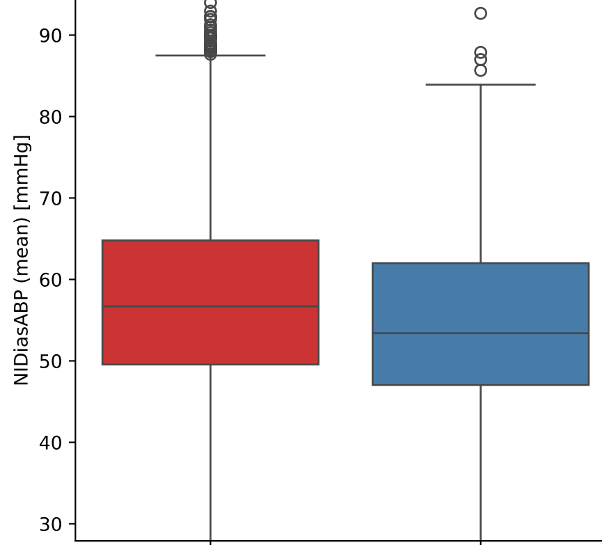
NIDiasABP (mean) vs Outcome
