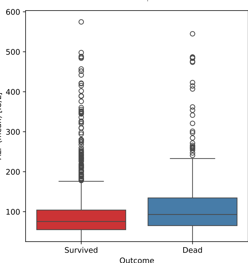
ALP (mean) vs Outcome
