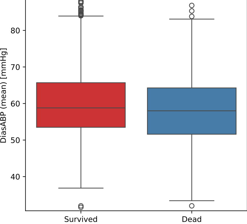
DiasABP (mean) vs Outcome
