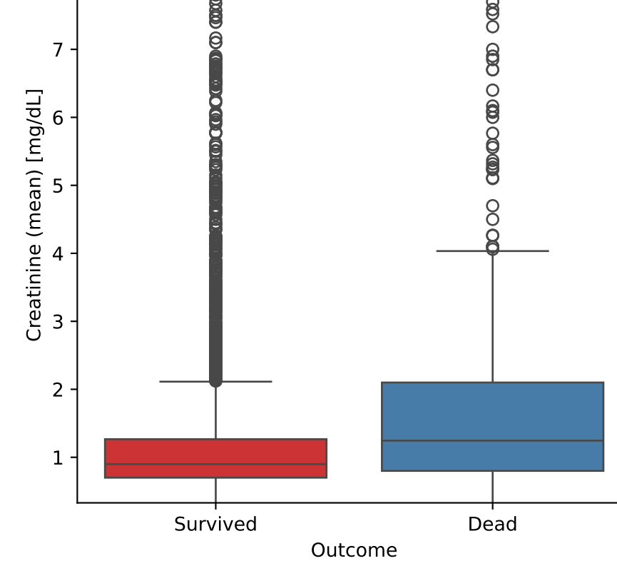
Creatinine (mean) vs Outcome
