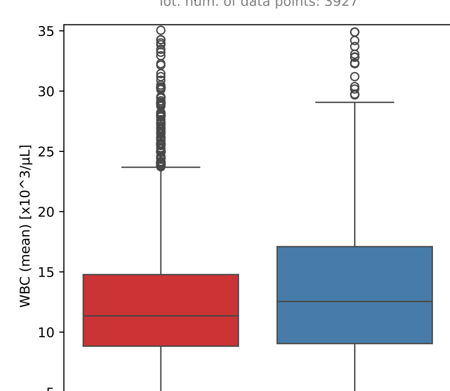
WBC (mean) vs Outcome
