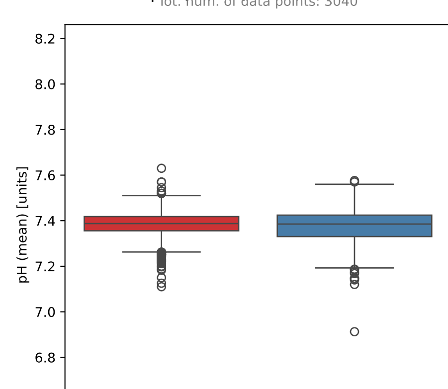
pH (mean) vs Outcome
