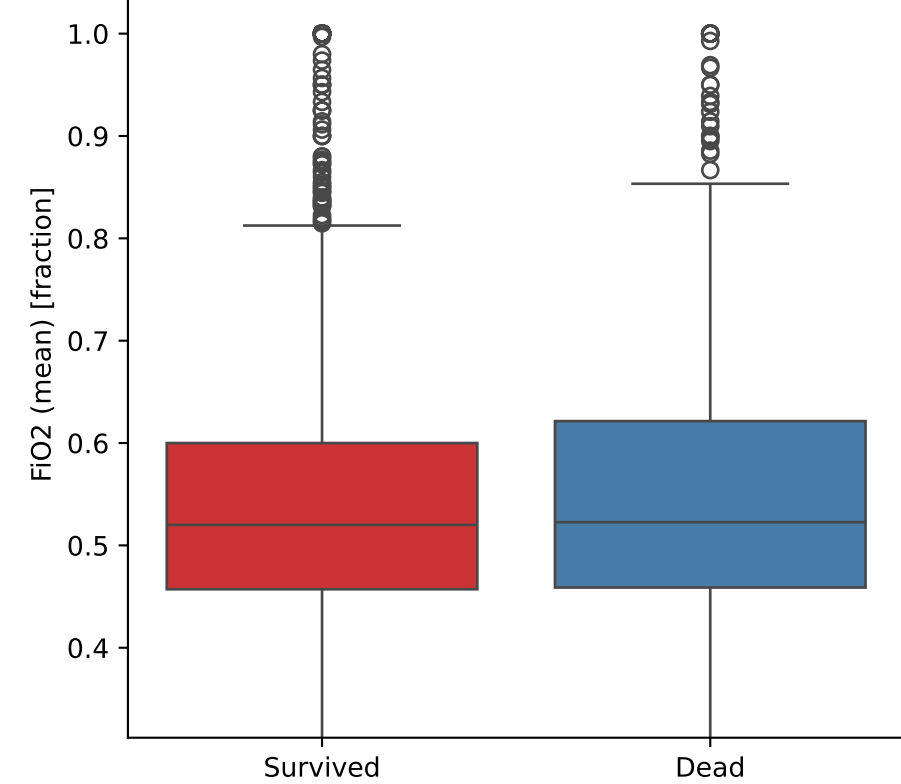
FiO2 (mean) vs Outcome
