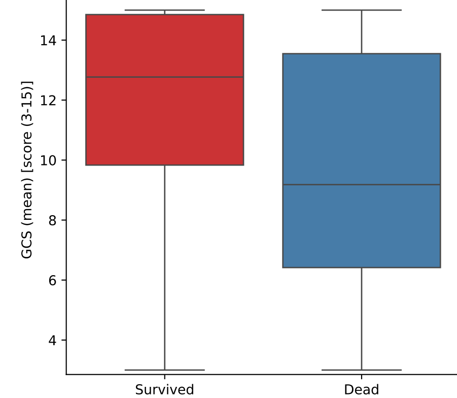
GCS (mean) vs Outcome
