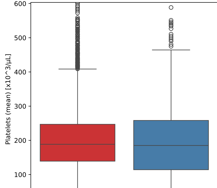
Platelets (mean) vs Outcome
