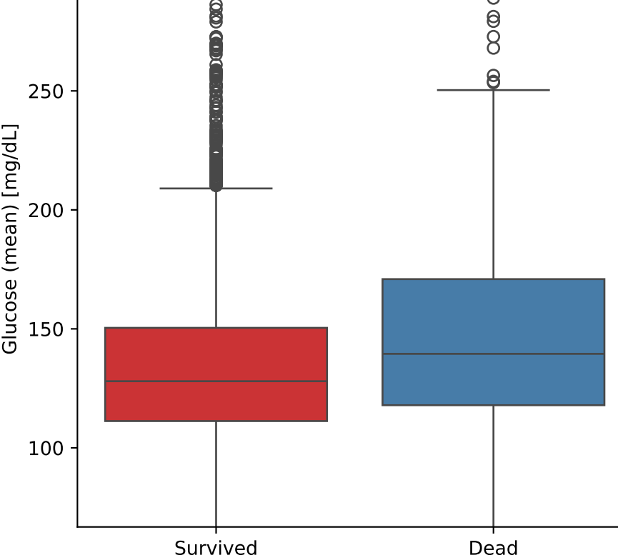
Glucose (mean) vs Outcome
