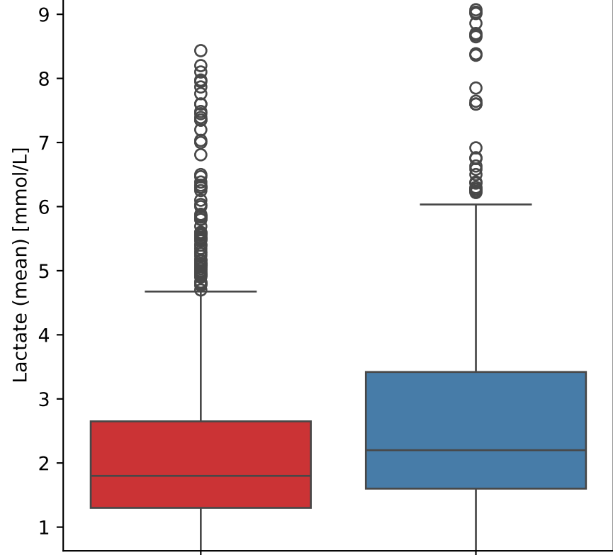
Lactate (mean) vs Outcome
