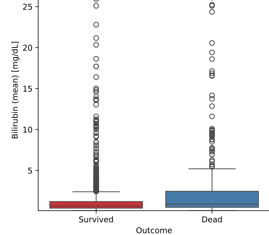
Bilirubin (mean) vs Outcome
