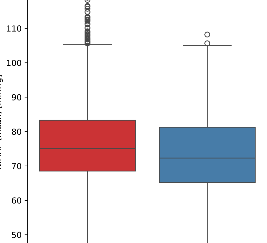
NIMAP (mean) vs Outcome
