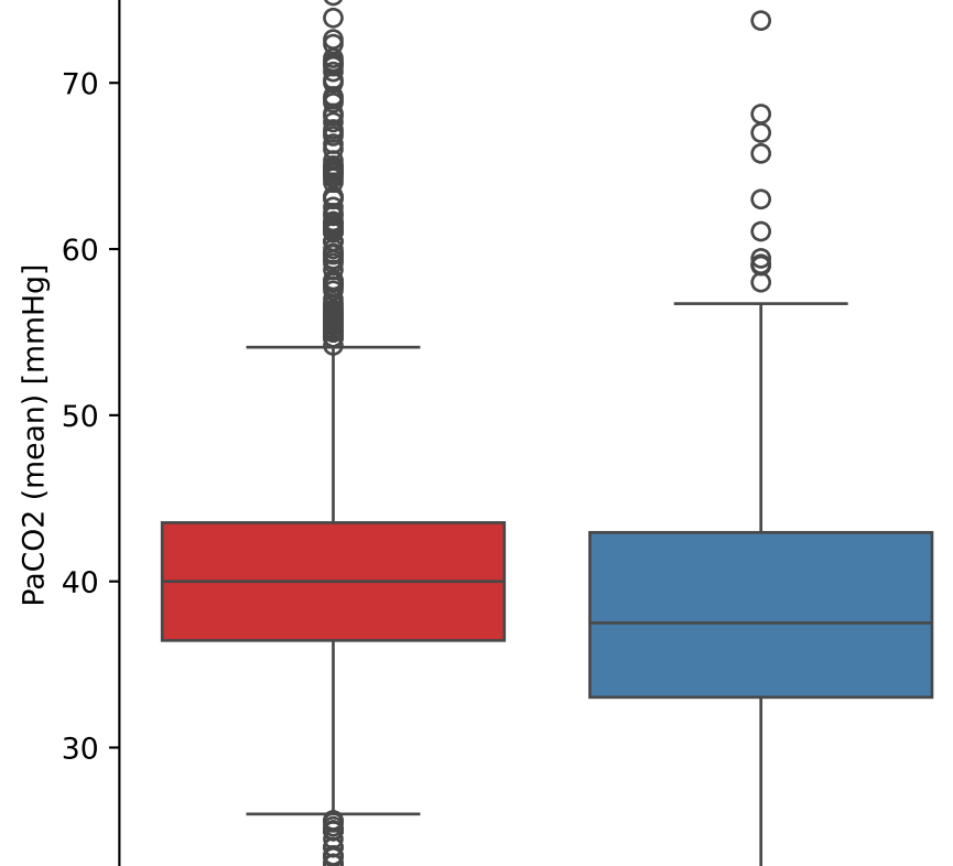
PaCO2 (mean) vs Outcome
