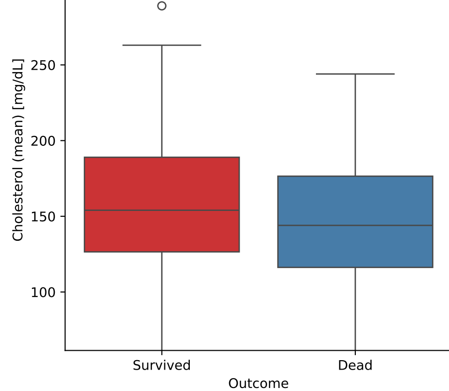
Cholesterol (mean) vs Outcome
