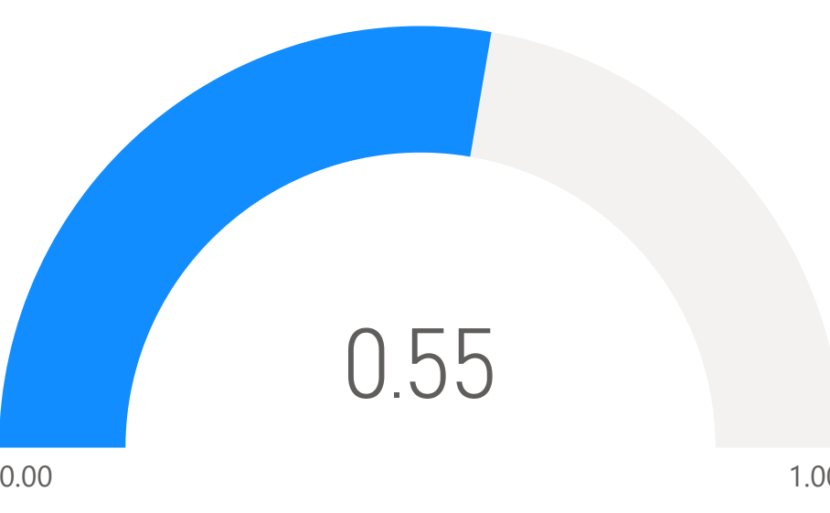
AdaBoost Recall
