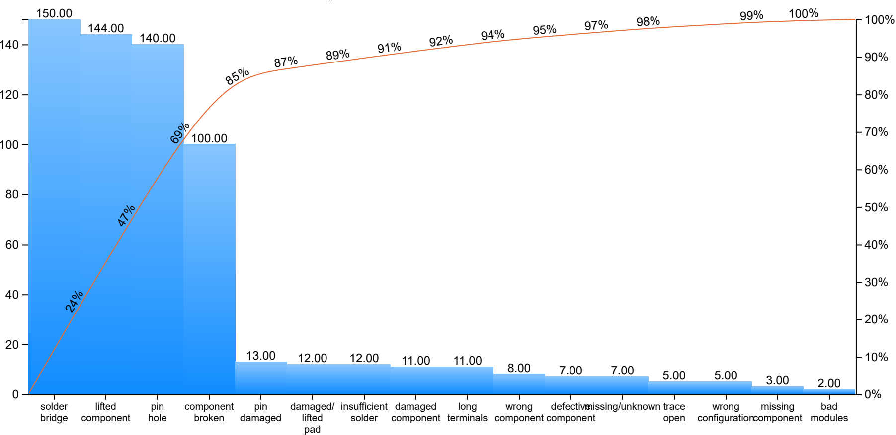
Defect Frequencies for Production Model 595130
