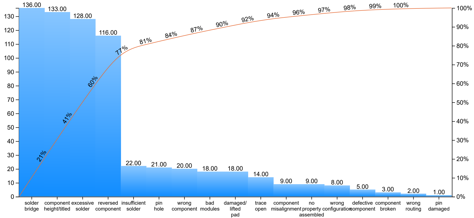
Defect Frequencies for Model 595214
