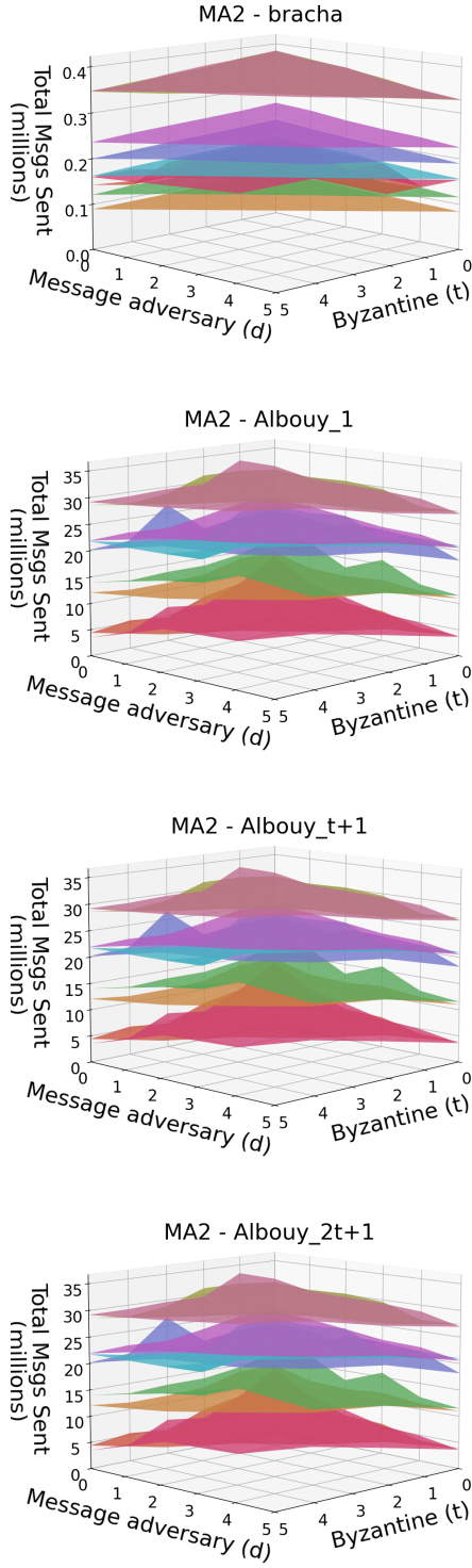
Fig. 9: 3D Plots comparing the tot_MSGS of the four algorithms (Bracha, Albouy_1, Albouy_t+1 and Albouy_2t+1) across all topology when varying (t, d) and considering MA2.
