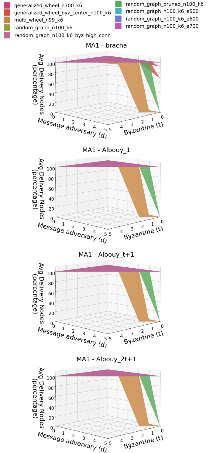
Fig. 3: 3D Plots comparing the avg_CND of the four algorithms (Bracha, Albouy_1, Albouy_t+1 and Albouy_2t+1) across all topology when varying (t, d) and considering MA1
