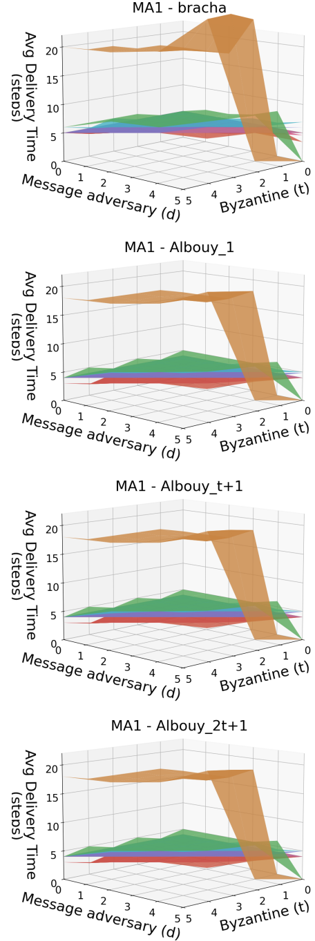
Fig. 4: 3D Plots comparing the \text{avg\_TTD} of the four algorithms (Bracha, Albouy_1, Albouy_t+1 and Albouy_2t+1) across all topology when varying (t, d) and considering MA1.
