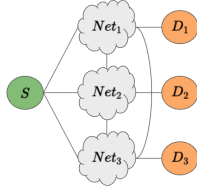
Fig. 2: Illustration of the network G with n = 3(t+2d+x)+1 nodes, \alpha = 3 and connectivity k(G) \geq t+d+x . The orange sets D_i represent the groups of correct nodes that the message adversary MA1(d) can isolate by blocking communications from any p \in Net_i to every q \in D_i .
