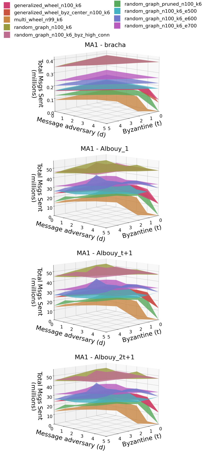
Fig. 5: 3D Plots comparing the tot_MSGS of the four algorithms (Bracha, Albouy_1, Albouy_t+1 and Albouy_2t+1) across all topology when varying (t, d) and considering MA1.
