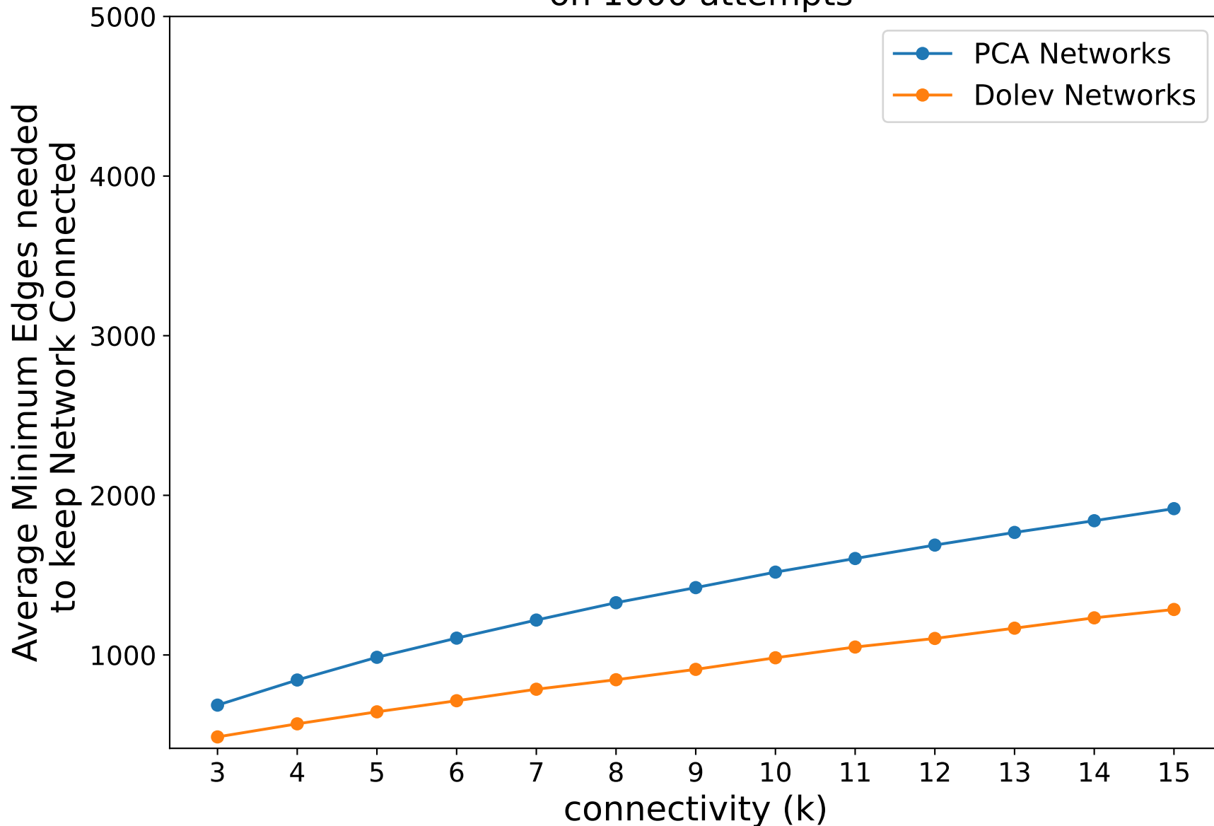
Edge Removal Inverse Comparison for a network of n=100 nodes on 1000 attempts
