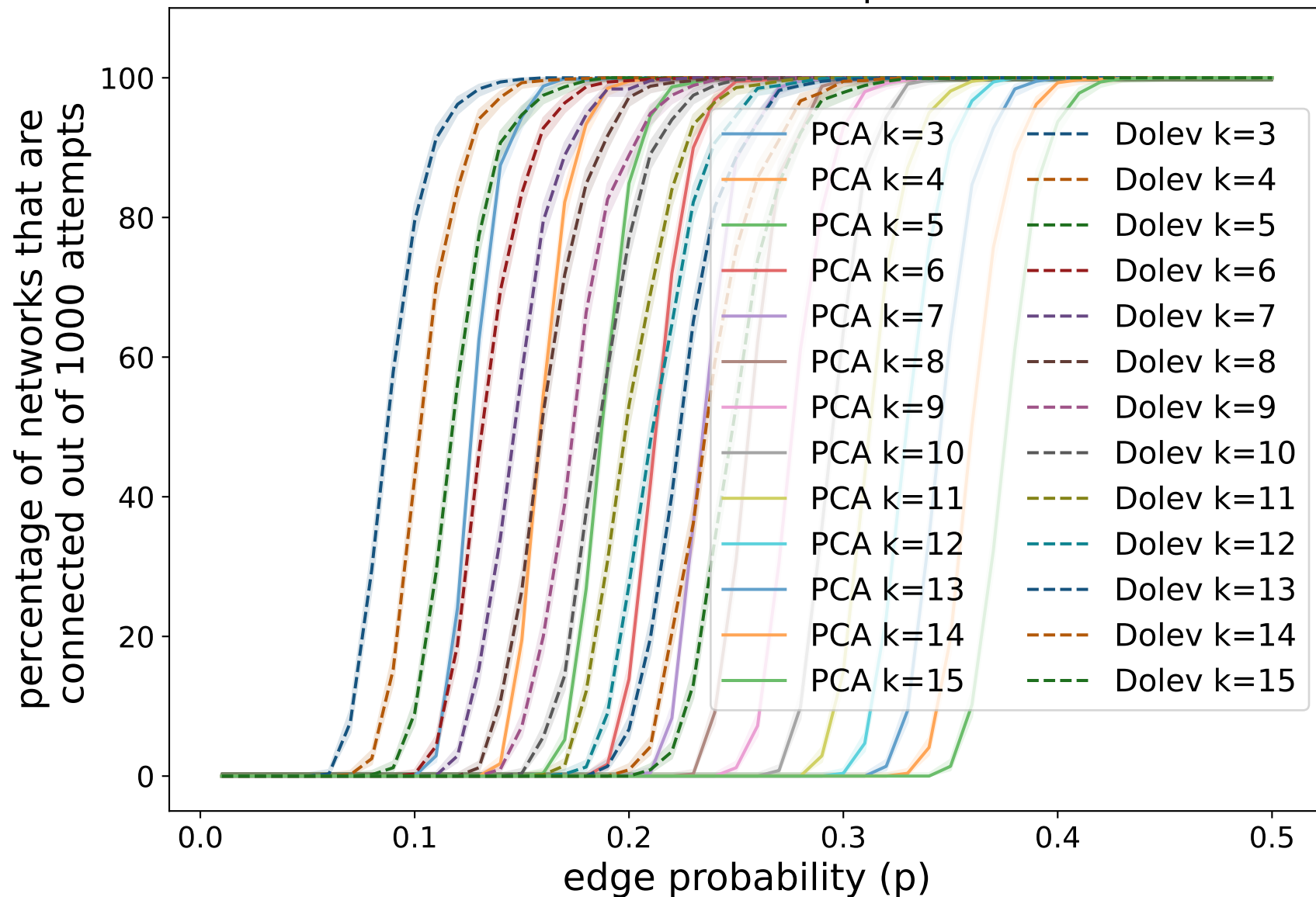
Erdos Renyi Comparison for a network of n=100 nodes on 1000 attempts
