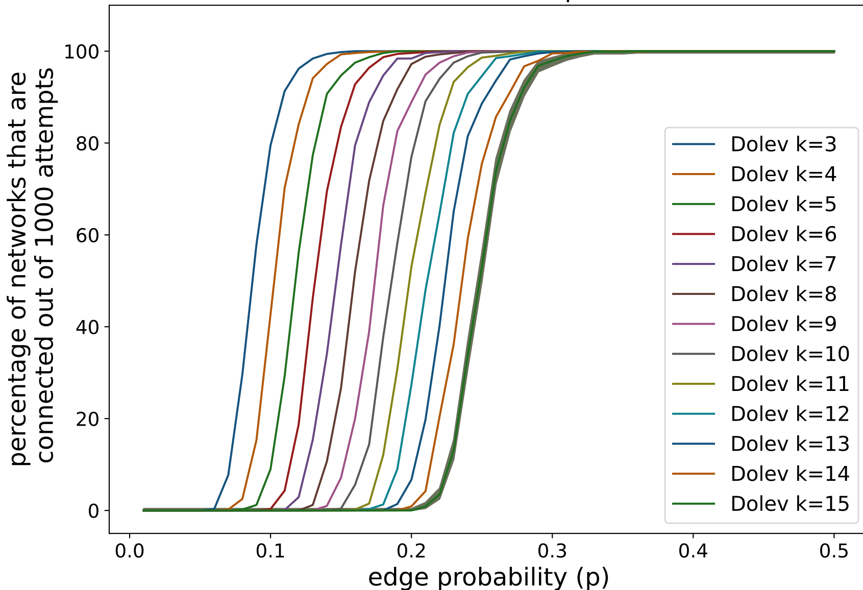
[DOLEV] Erdos Renyi Comparison for a network of n=100 nodes on 1000 attempts
