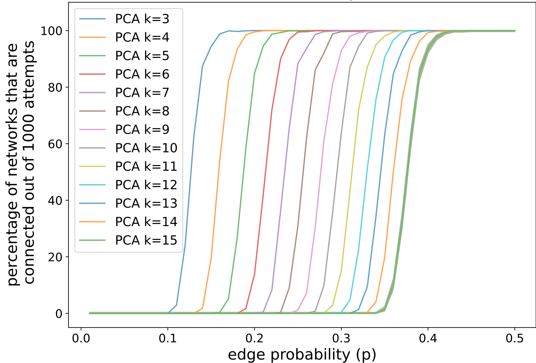
[PCA] Erdos Renyi Comparison for a network of n=100 nodes on 1000 attempts
