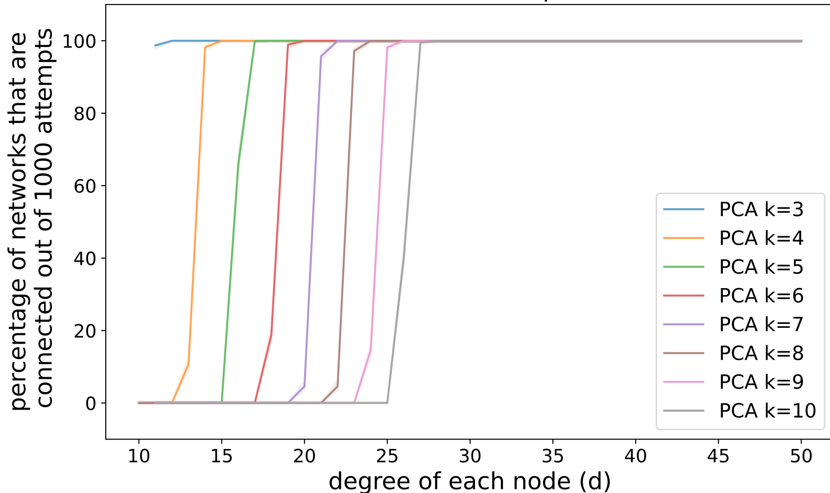
[PCA] Random Regular Comparison for a network of n=100 nodes on 1000 attempts
