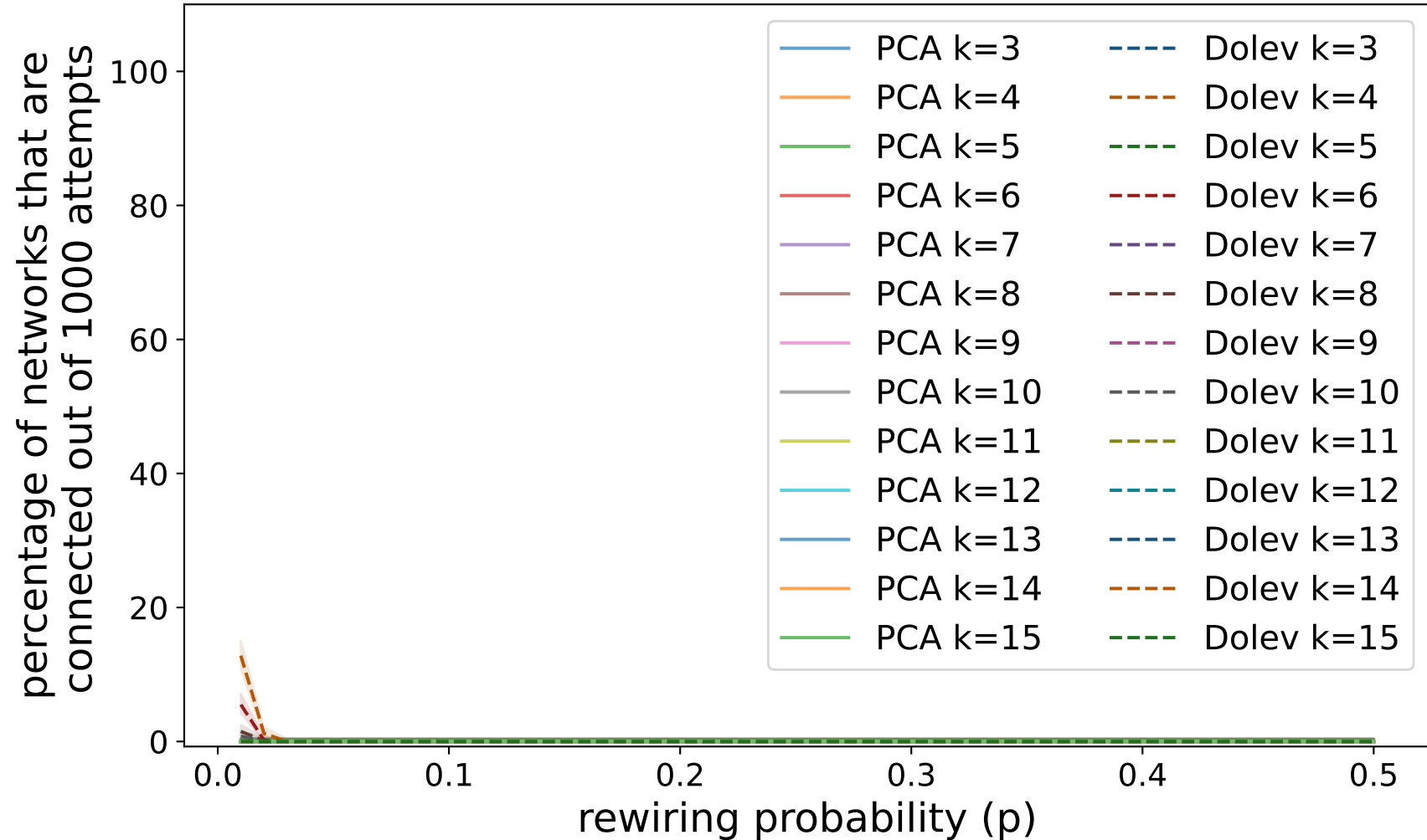
Watts Strogatz Comparison for a network of n=100 nodes on 1000 attempts
