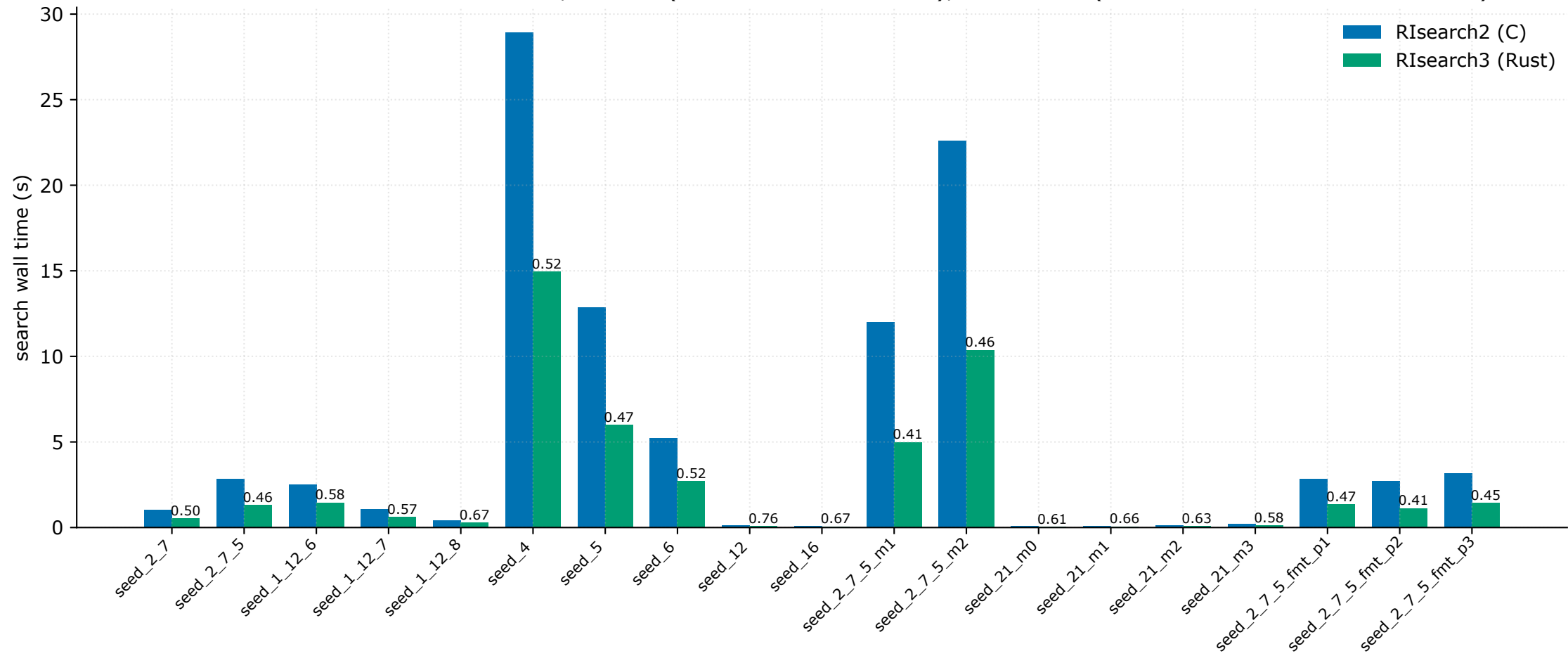
RIsearch2 vs RIsearch3 search time, ext=20 (seed 21 mm=0: ext=0), 32 threads (labels: time relative to RIsearch2)
