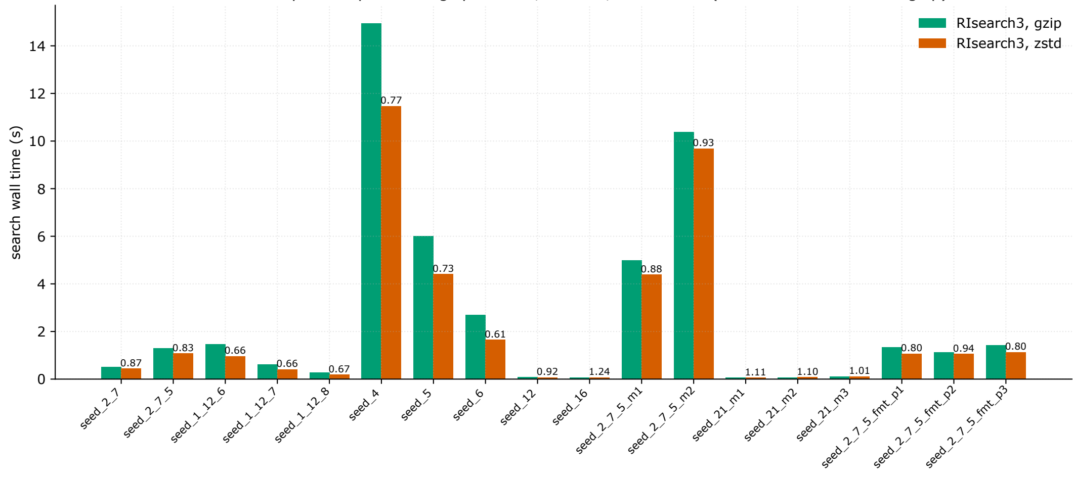
RIsearch3 output compression: gzip vs zstd, ext=20, 32 threads (labels: time relative to gzip)
