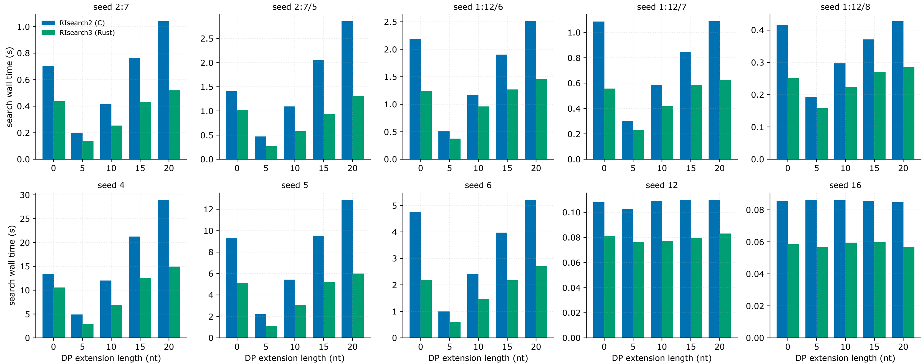
Search time vs extension length, 32 threads
