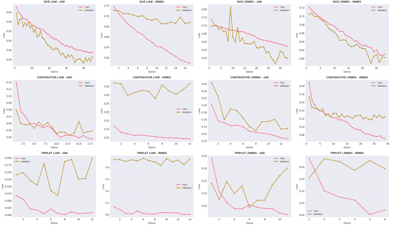
Fig. A4 Training and validation loss curves, ResNet-18, all 12 loss×split combinations.
