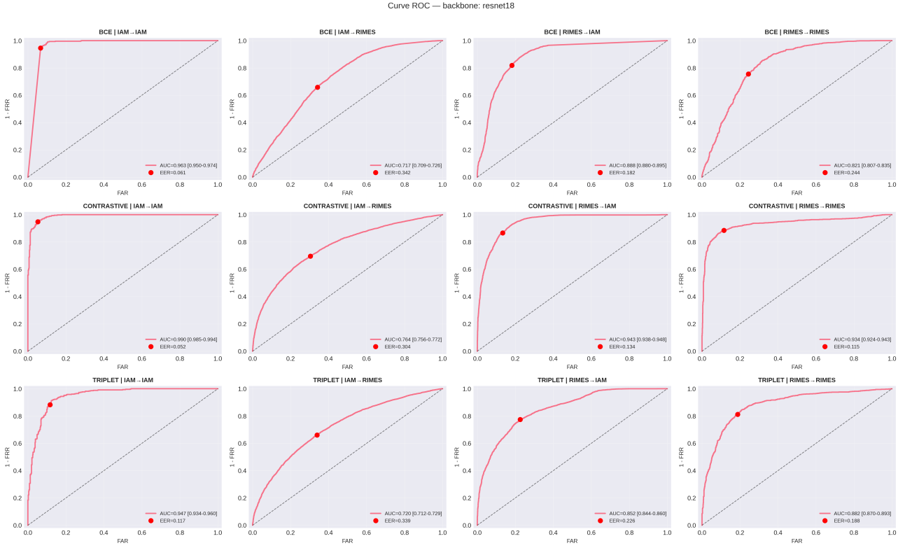
Fig. 7 ROC curves, ResNet-18, all losses/splits. Bootstrap 95% confidence intervals for AUC are reported in each panel legend.
