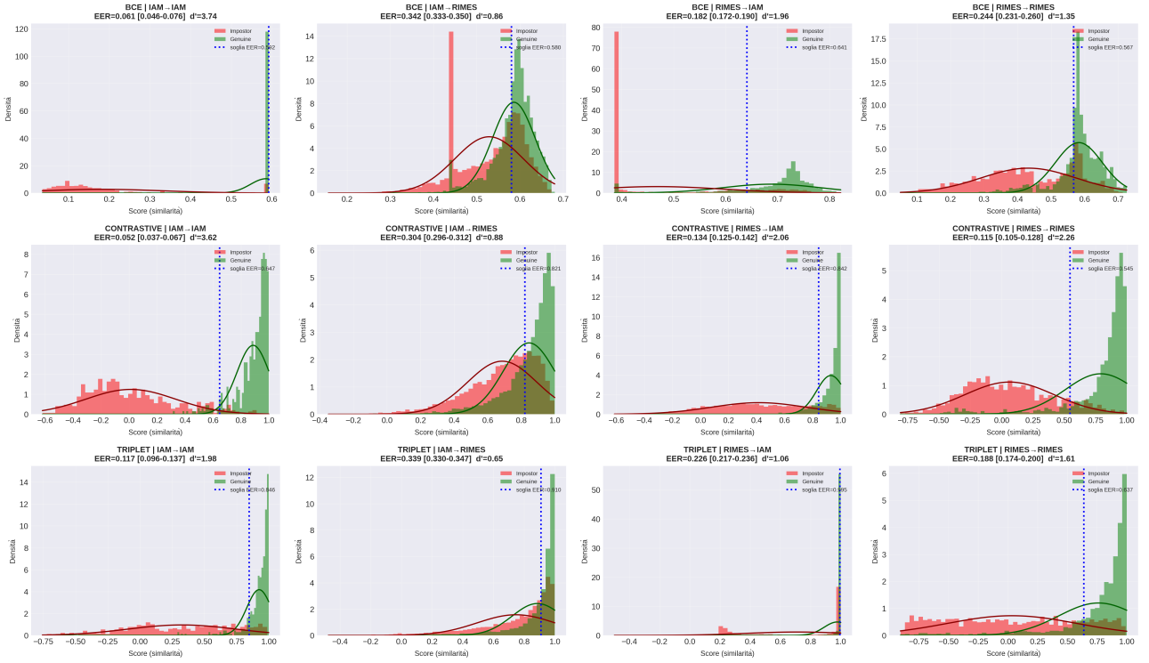
Fig. 9 Genuine (green)/impostor (red) scores with fitted Gaussian overlays, ResNet-18, all loss×split combinations. Dotted lines: EER threshold. None of the 12 distributions shown pass Shapiro–Wilk at \alpha = 0.05 .
