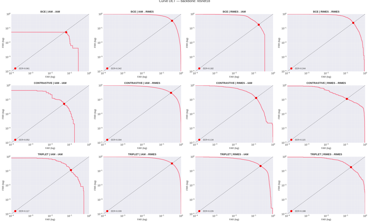
Fig. 8 DET curves (log-log), ResNet-18, all losses/splits.
