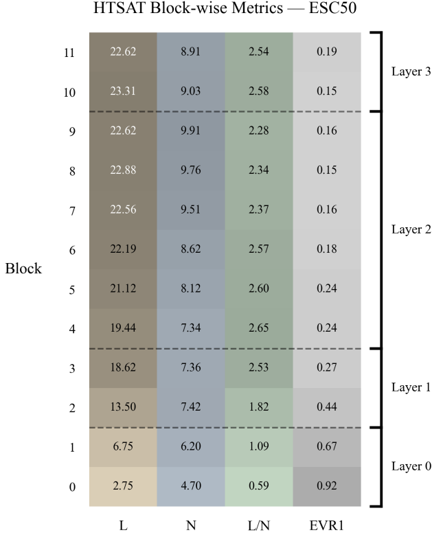
Figure 3. Block-wise metrics for the ESC-50 dataset. The heatmap shows the per-block average (blocks 0–11) of linear dimensionality ( L with \alpha = 0.99 ), nonlinear dimensionality ( N ), the L/N ratio, and the dominance of the first principal component (EVR 1 ). Dashed lines separate the four stages (Layers 0–3) of the architecture.
