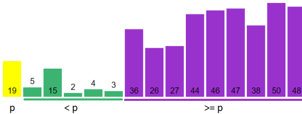
Figure 2.1: Sorting Visualization, Example of First Partition of Quick Sort
