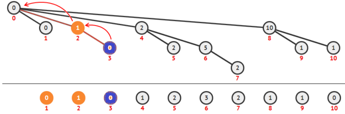
Figure 2.13: Example of \text{rsq}(3) on Fenwick (Interrogation/Query) Tree
