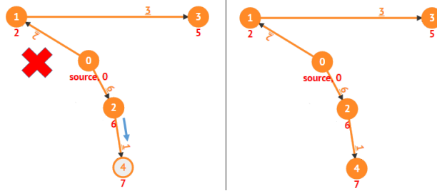
Figure 4.18: Dijkstra's Animation, Steps 5+6
