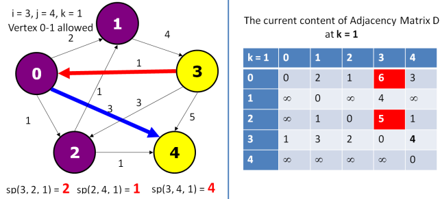
Figure 4.25: Floyd-Warshall Explanation 3
