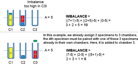
Figure 3.8: UVa 00410 - Observations
