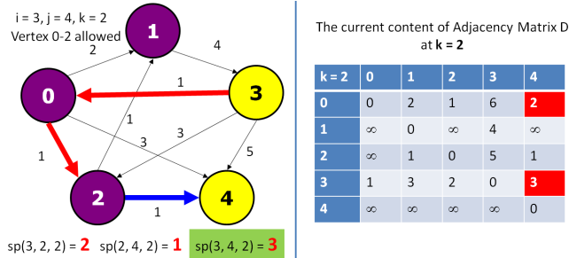
Figure 4.26: Floyd-Warshall Explanation 4
