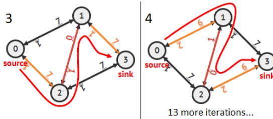
Figure 8.13: Illustration of Ford-Fulkerson Method (DFS)—Part 2
