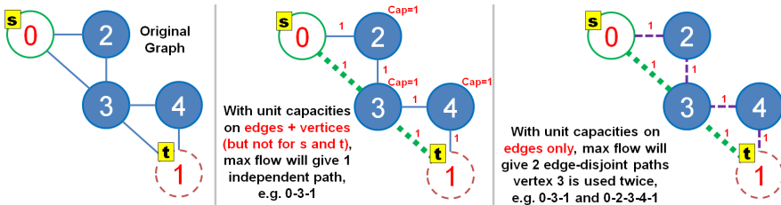
Figure 8.20: Comparison Between Max Independent Paths vs Max Edge-Disjoint Paths
