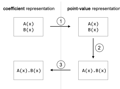
Figure 9.11: Fast polynomial multiplication: The big idea
