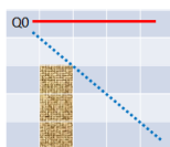
Figure 8.2: 5-Queens problem; After placing the first Queen
