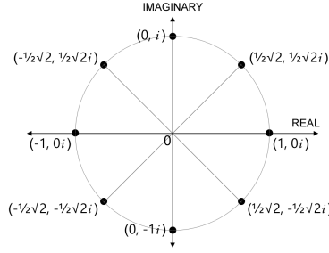
Figure 9.12: The 8 th roots of unity.
