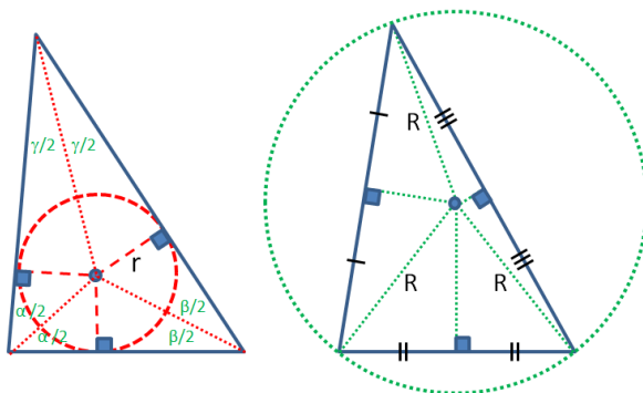
Figure 7.6: Incircle and Circumcircle of a Triangle
