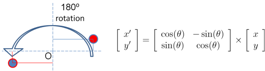
Figure 7.1: Rotating the point (10, 3) by 180^\circ counterclockwise around the origin (0, 0)
