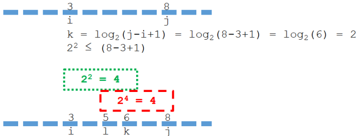
Figure 9.1: Explanation of an Example \text{RMQ}(i, j)
