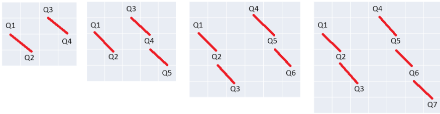
Figure 9.36: Stair-Step Pattern for Small N -Queens Instances
