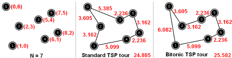
Figure 8.25: The Standard TSP versus Bitonic TSP
