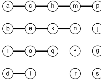
Figure 9.3: Heavy-Paths of the Tree in Figure 9.2
