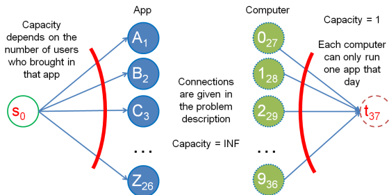
Figure 8.18: Residual Graph of UVa 00259 [28]
