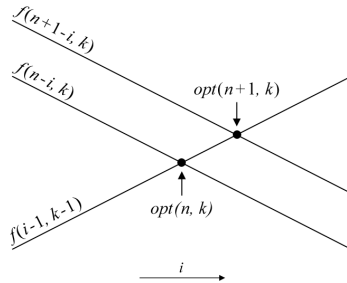
Figure 9.14: opt(n, k) vs. opt(n+1, k)
