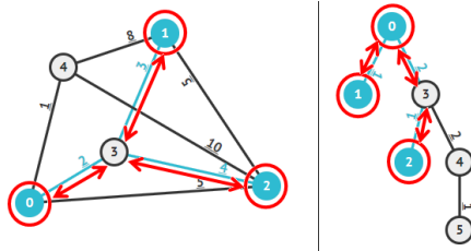
Figure 8.35: Steiner Tree Illustrations—Part 2
