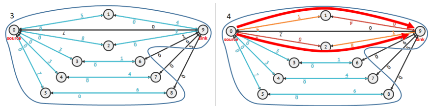
Figure 8.16: Illustration of Dinic's Algorithm (BFS)—Part 2
