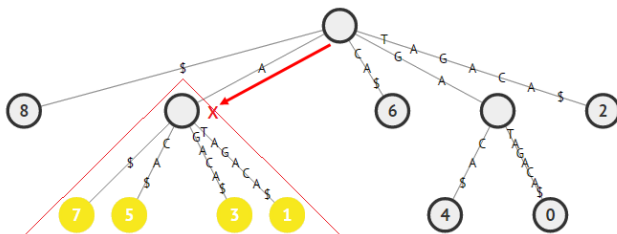
Figure 6.4: String Matching of T = \text{"GATAGACAS\$"}^14 with Pattern String P = \text{"A"}^15
