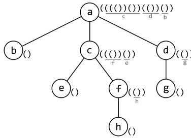
Figure 9.8: Example of Rooted Tree Encoding with Bracket Tuples.
