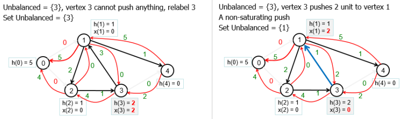
Figure 9.21: Left: Relabel Vertex 3; Right: Non-saturating Push 3 \rightarrow 1
