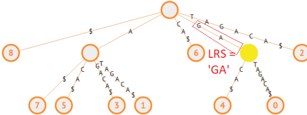
Figure 6.5: Longest Repeated Substring of T = \text{"GATAGACA\$"}^2
