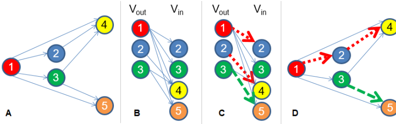
Figure 8.32: Min Path Cover on DAG (from UVa 01201 [28])
