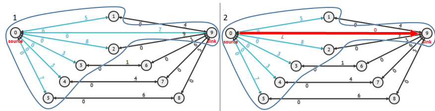
Figure 8.15: Illustration of Dinic's Algorithm (BFS)—Part 1
