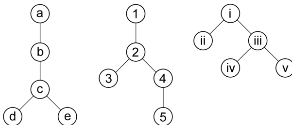
Figure 9.5: Three Isomorphic Trees.
