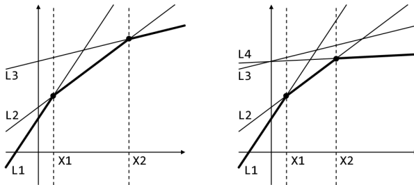
Figure 9.15: The bolded line is the convex line which gives the minimum y for a given x .
