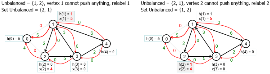
Figure 9.18: Left: Relabel Vertex 1; Right: Relabel Vertex 2
