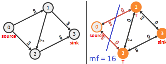
Figure 8.11: Max Flow/Min Cut Illustration
