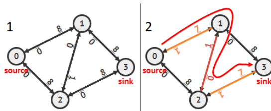
Figure 8.12: Illustration of Ford-Fulkerson Method (DFS)—Part 1
