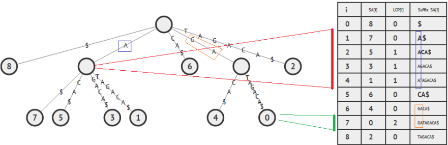
Figure 6.8: Suffix Tree (Left) and Suffix Array (Right) of T = \text{"GATAGACA\$"}
