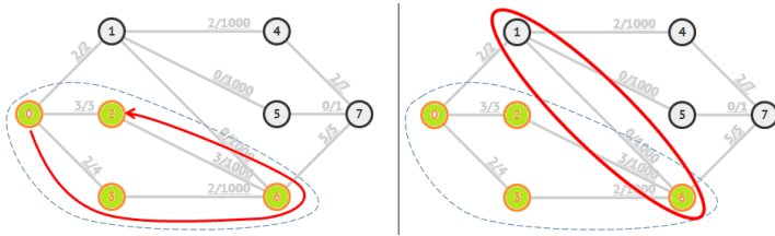
Figure 8.30: König's Theorem for MWVC Variant
