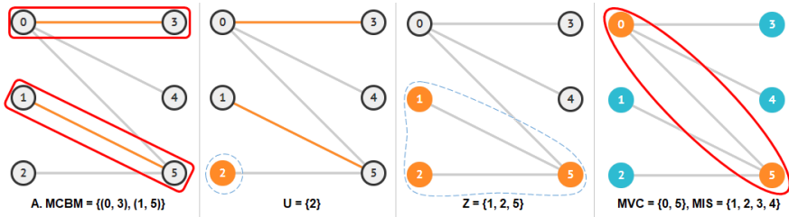
Figure 8.28: MCBM and König's Theorem
