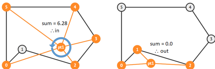
Figure 7.11: Left: Inside Polygon, Right: Outside Polygon
