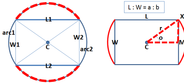
Figure 8.37: Athletics Track (from UVa 11646)
