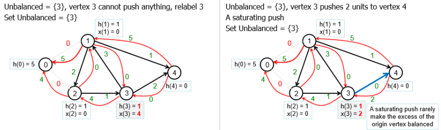
Figure 9.20: Left: Relabel Vertex 3; Right: Saturating Push 3 \rightarrow 4
