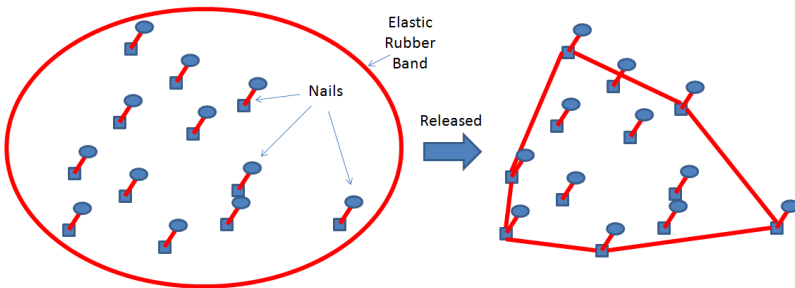
Figure 7.13: Rubber Band Analogy for Finding Convex Hull
