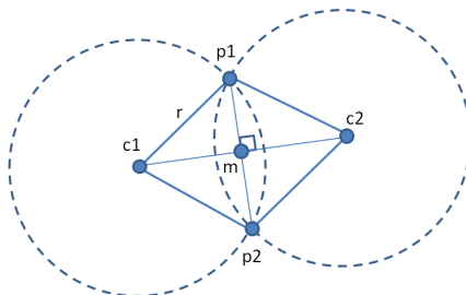
Figure 7.4: Explanation for Circle Through 2 Points and Radius
