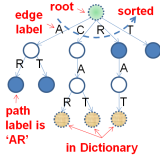
Figure 6.2: Suffix Trie
