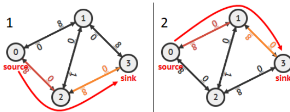
Figure 8.14: Illustration of Edmonds-Karp Algorithm (BFS)
