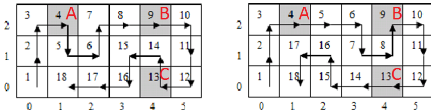
Figure 8.26: Visualization of UVa 01098 - Robots on Ice
