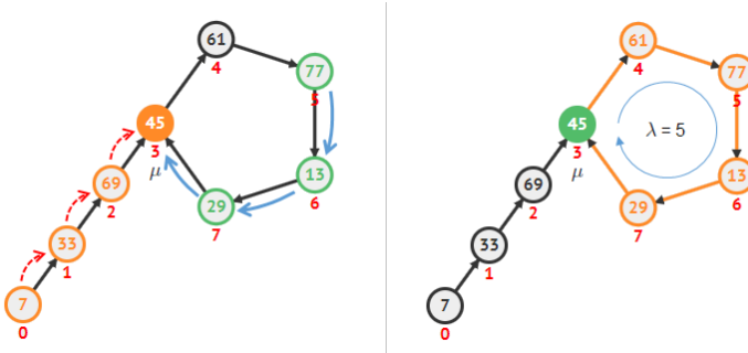
Figure 5.4: Left: Finding \mu = 3 ; Right: Finding \lambda = 5
