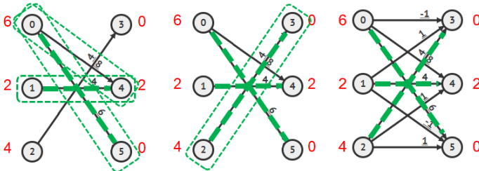
Figure 9.27: L+M: 2nd+3rd Augmenting Paths; R: Max Weighted Perfect Matching
