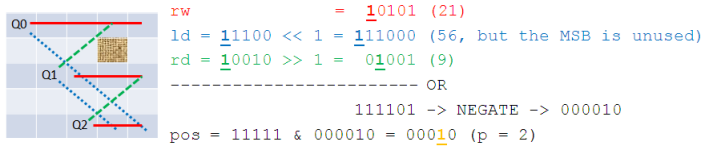
Figure 8.4: 5-Queens problem; After placing the third Queen
