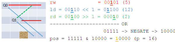
Figure 8.3: 5-Queens problem; After placing the second Queen
