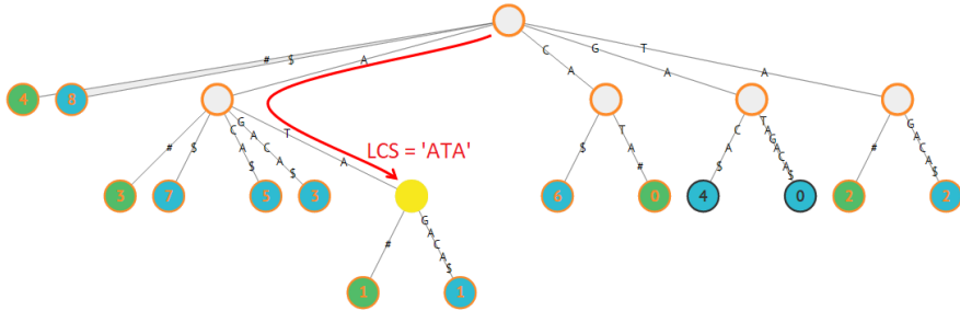
Figure 6.6: Generalized ST of T_1 = \text{"GATAGACA\$"}^3 and T_2 = \text{"CATA\#"} and their LCS
