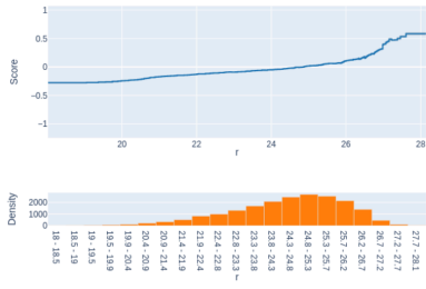
Term: r (continuous)
