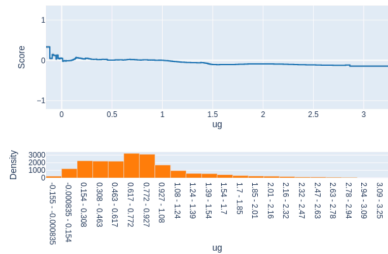
Term: ug (continuous)
