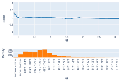
Term: ug (continuous)
