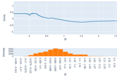
Term: gr (continuous)
