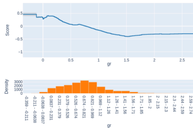
Term: gr (continuous)
