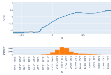
Term: zy (continuous)
