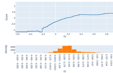
Term: zy (continuous)
