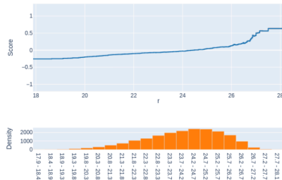
Term: r (continuous)
