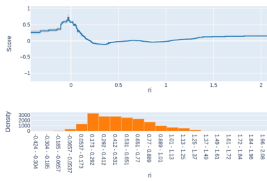
Term: ri (continuous)
