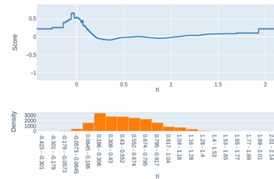
Term: ri (continuous)
