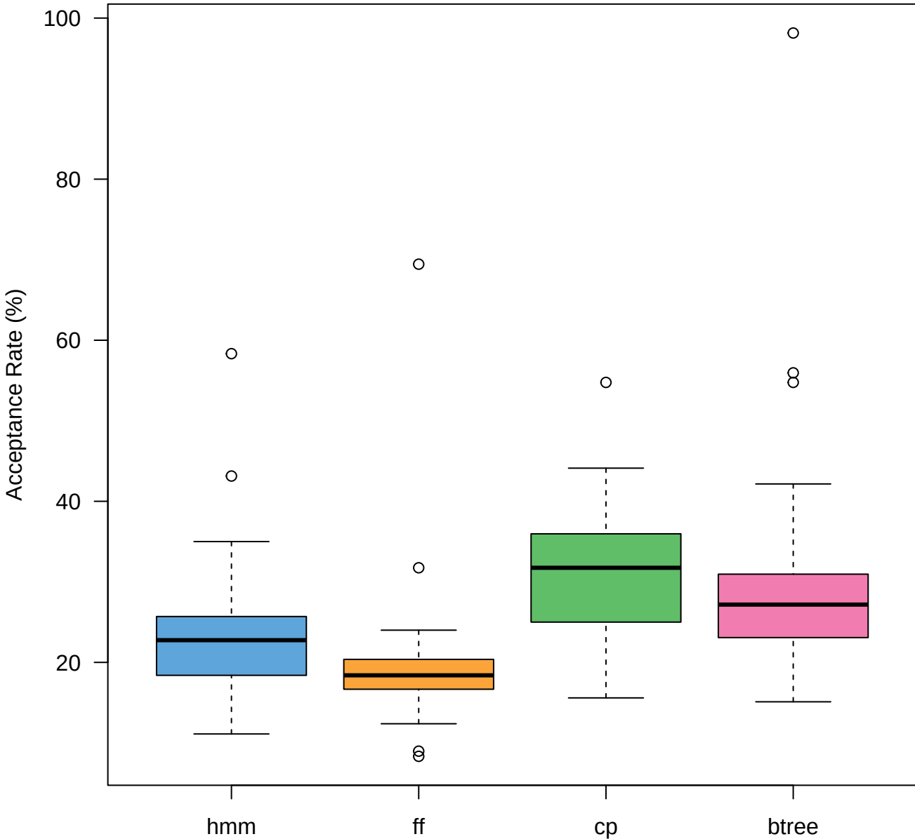
Speculative Decoding Acceptance Rates by Model
