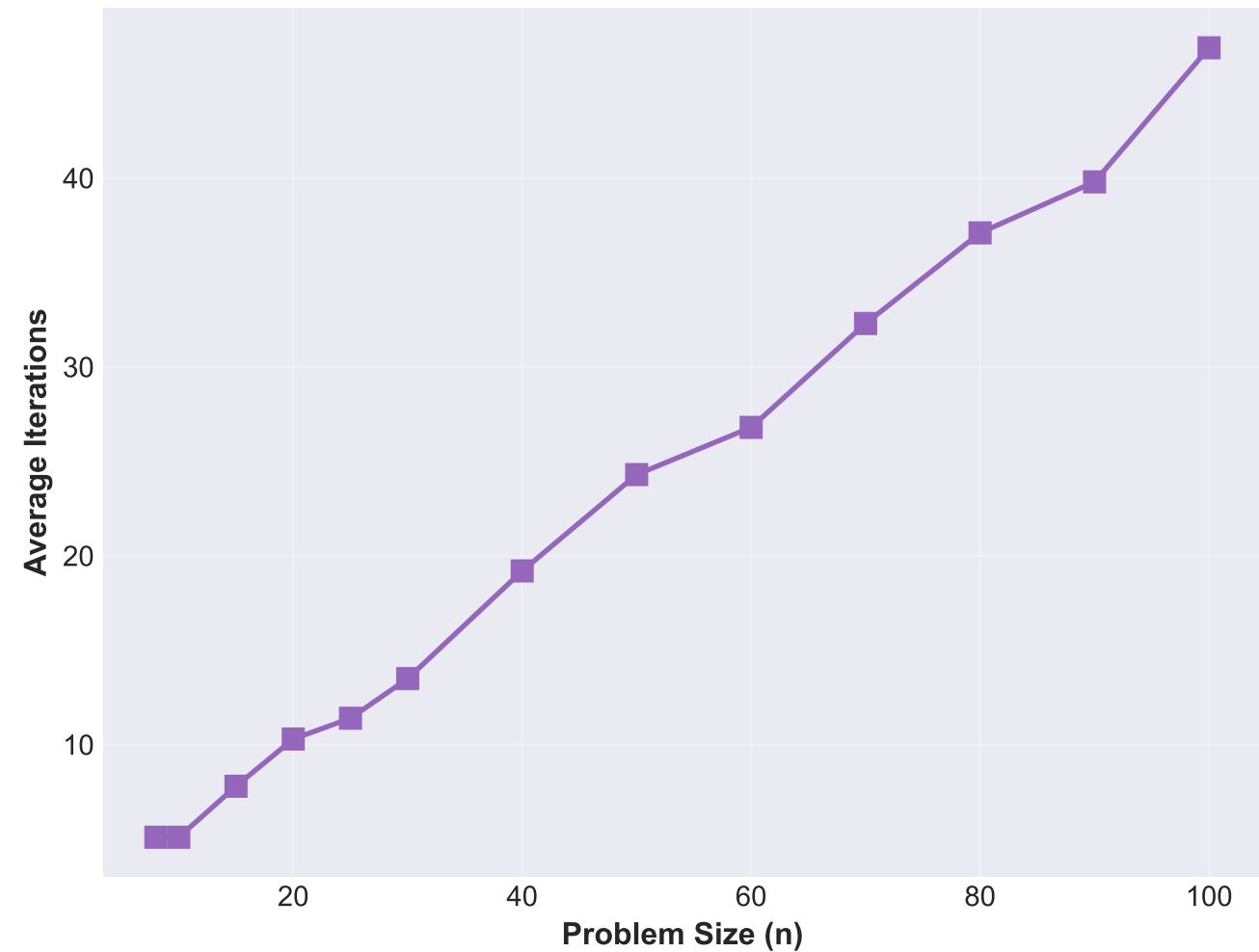
Iteration Count
