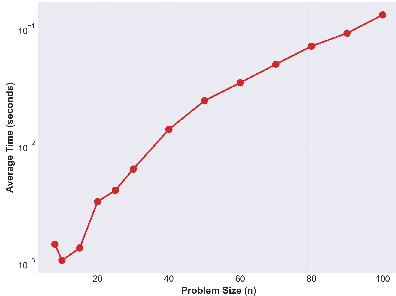
Execution Time
