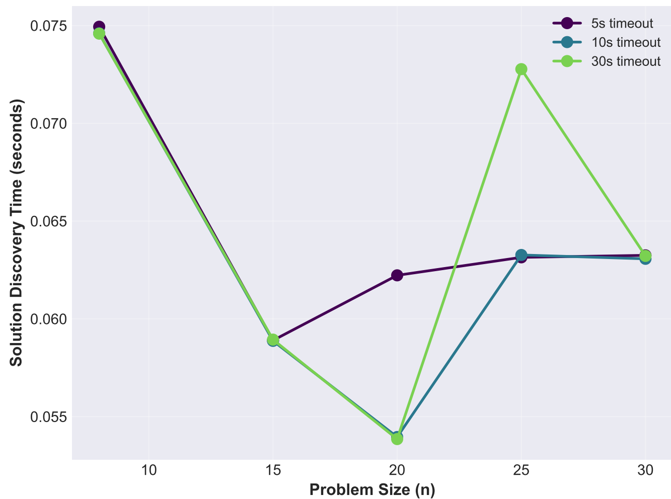
Solution Time vs Timeout
