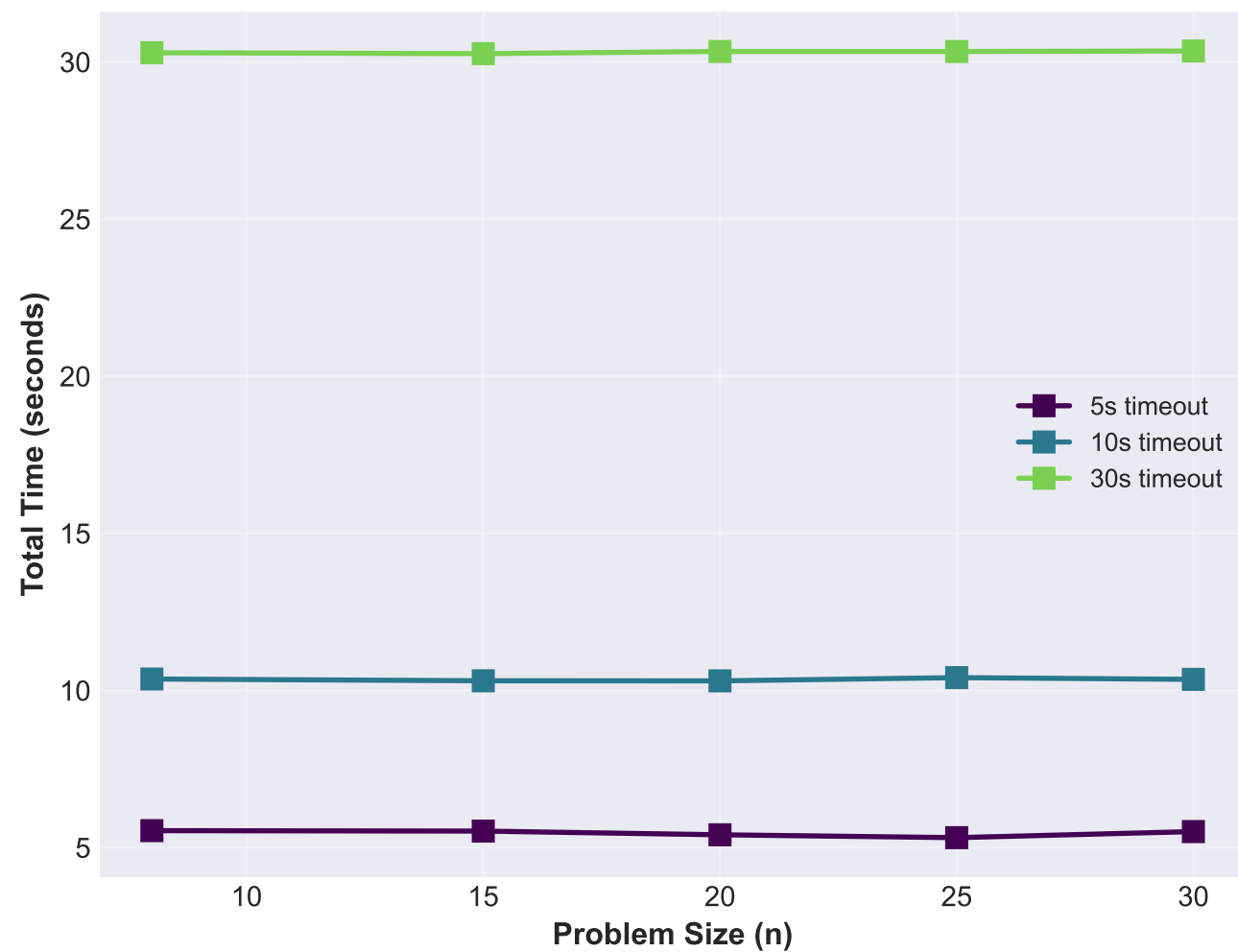
Total Time vs Timeout
