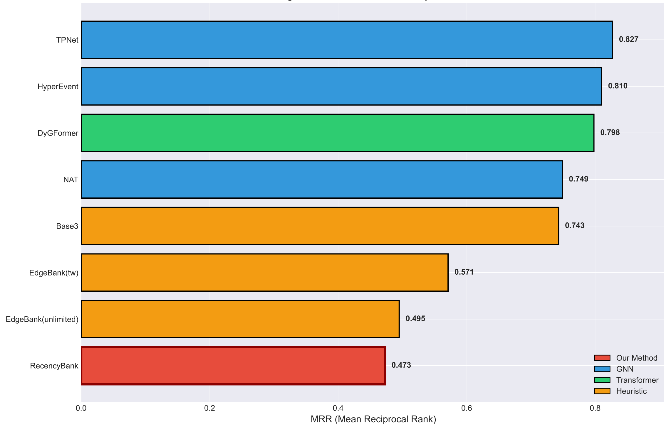
tgbl-wiki Leaderboard Comparison
